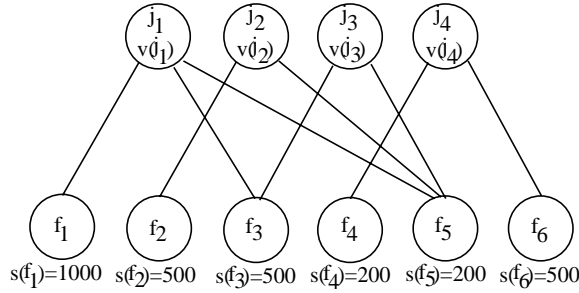
Figure 1: A bipartite graph depiction of a set of jobs and their file requests.
