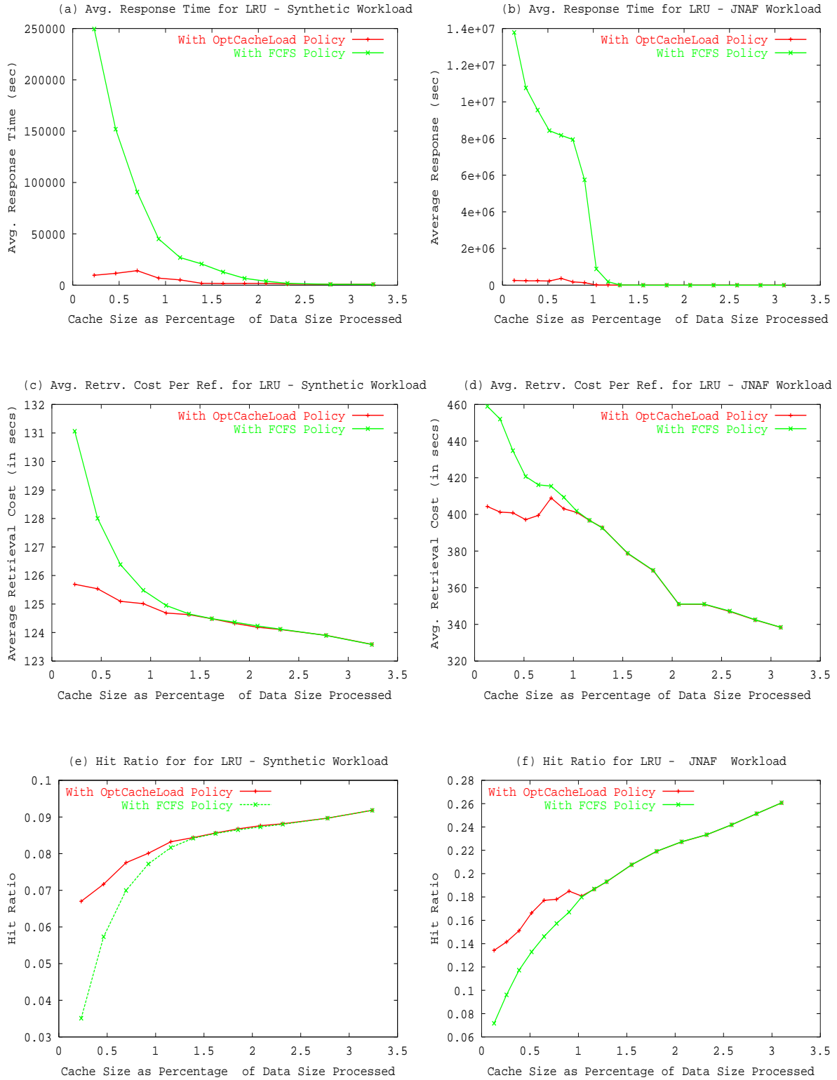
Figure 5: Effect of OptCacheLoad on Jobs Serviced at an SRM using LRU Cache Replacement Algorithm
