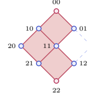
(b) A cubic realization of a subset of the 2^\omega -cliffs of order 2.
