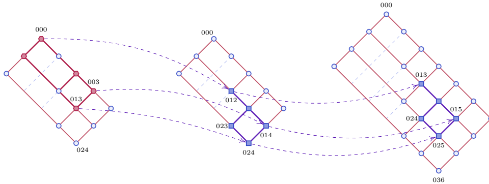
Figure 2.8: From the top to bottom and left to right, here are the posets \text{Ca}_2(3) , \text{Ca}_2(3) , and \text{Ca}_3(3) . The two last posets contain \mathcal{I}(\text{Hi}_1)(3) as subposets. There is a poset morphism between the output-wings of the first one and the input-wings of the second one.
