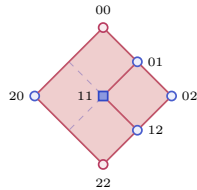
(c) A cubic realization of a subset of the 2^\omega -cliffs of order 2.
