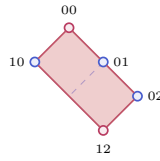
(a) A cubic realization of a subset of the 2^\omega -cliffs of order 2.
