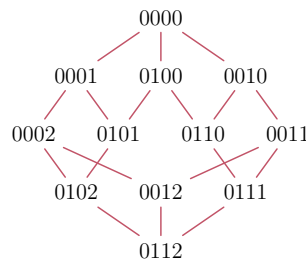
Figure 1.2: The Hasse diagram of the poset (\text{Cl}_{0112^\omega}(4), \preceq') .
