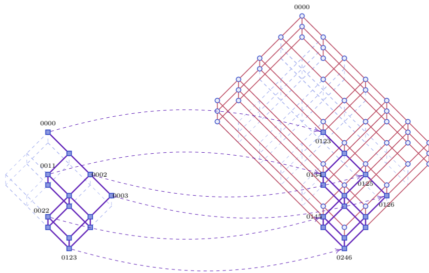
Figure 2.10: The subset of Ca_2(4) formed by its input-wings is isomorphic to Hi_1(4) .
