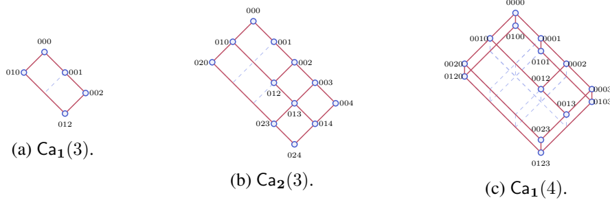
Figure 2.5: Hasse diagrams of some \delta -canyon posets.
