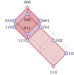
(d) A cubic realization of a subset of the 113^\omega -cliffs of order 3.
