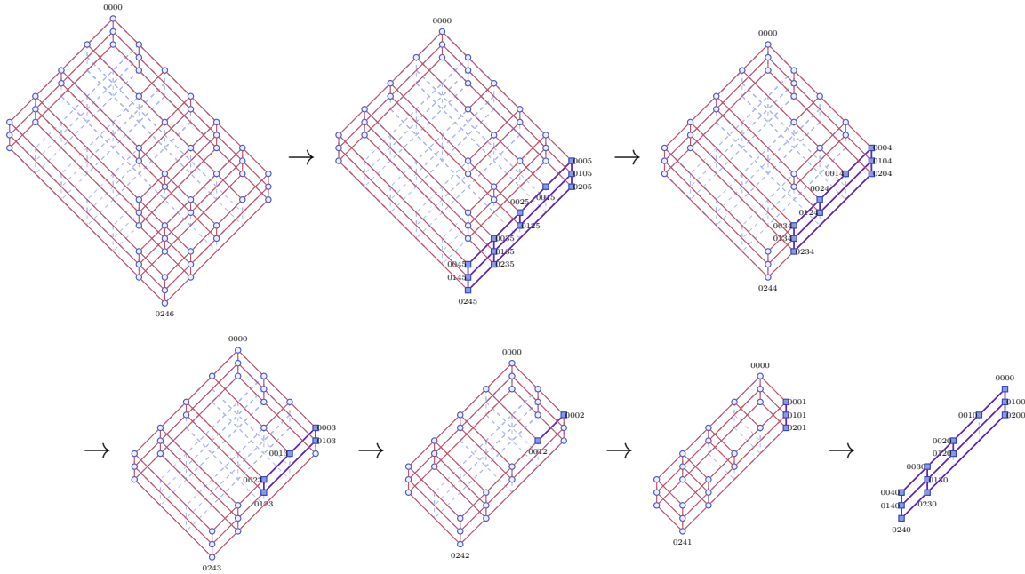
Figure 2.6: A sequence of interval contractions from \text{Ca}_2(4) to a poset isomorphic to \text{Ca}_2(3) . These interval contractions are poset derivations as introduced in Section 1.3.4. The marked intervals are the ones involved in the interval doubling operations.
