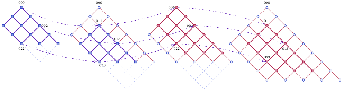
Figure 2.2: From the top to bottom and left to right, here are the posets \text{Av}_2(3) , \text{Av}_3(3) , \text{Av}_3(3) , and \text{Av}_4(3) . All these posets contain \text{Av}_2(3) as subposet by restricting on input-wings, output-wings, or butterflies.
