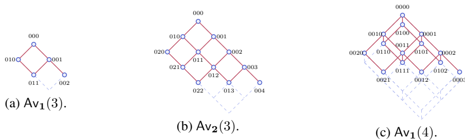
Figure 2.1: Hasse diagrams of some \delta -avalanche posets.
