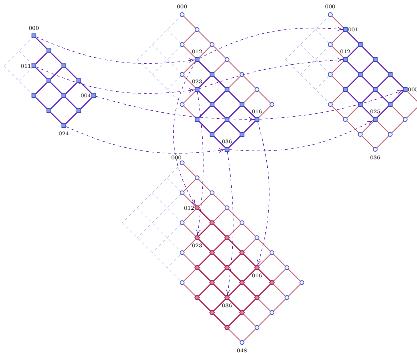
Figure 2.4: From the top to bottom and left to right, here are the posets \text{Hi}_2(3) , \text{Hi}_3(3) , \text{Hi}_3(3) , and \text{Hi}_4(3) . All these posets contain \text{Hi}_2(3) as subposet by restricting on input-wings, output-wings, or butterflies.
