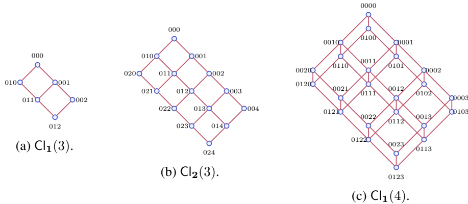
Figure 1.1: Hasse diagrams of some \delta -cliff posets.
