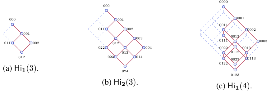
Figure 2.3: Hasse diagrams of some \delta -hill posets.
