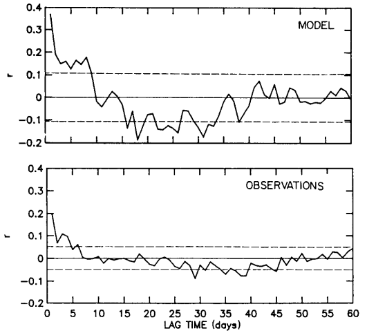
Fig. 12. Autocorrelation diagram of 1300 LT 222 Rn concentrations at Chester: normalized autocorrelation coefficient ( r ) versus time lag. Model results (top panel) are compared to observations (bottom panel). The dashed lines represent 95% confidence limits ( \pm 2/\sqrt{n} ; Chatfield, 1984).
