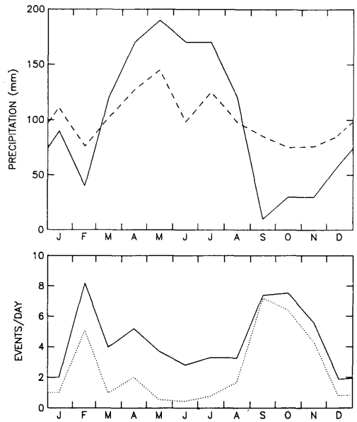
Fig. 9. Monthly total precipitation at Chester (top panel). The GCM results (solid line) are compared to mean observations for 1978–1984 (dashed line) as reported by Juzdan et al. (1985). The bottom panel shows monthly mean GCM frequencies of convective events in the Chester grid square column; sum of wet and dry convection (solid line) and dry convection only (dotted line). Convective events are recorded as hourly diagnostics, therefore the maximum frequency (corresponding to continuous convective mixing) is 24 events/day. Wet convection events are counted as half-events because only half of the lower gridbox is ventilated (see Section 2 of the text).
