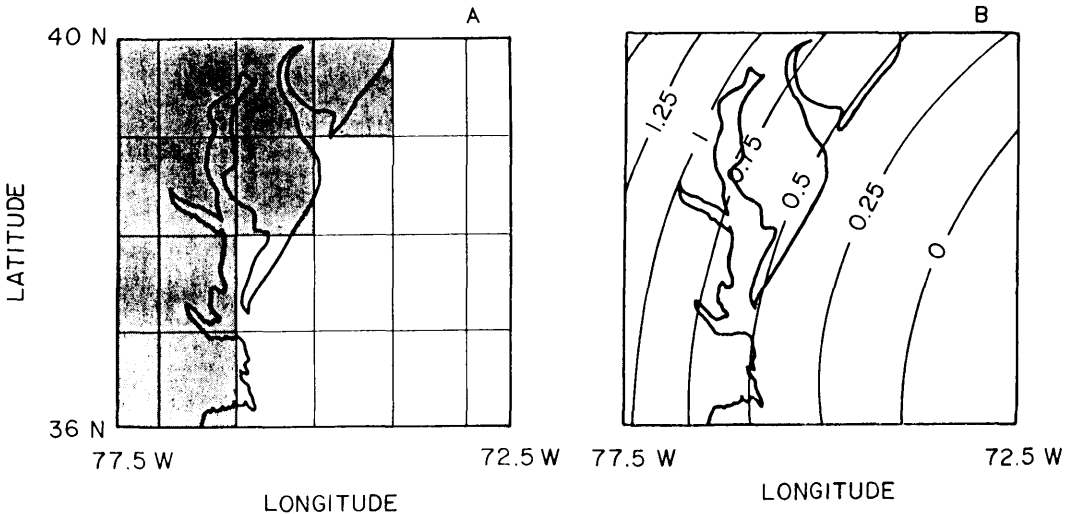
Fig. 3. (A) Land area (shaded) of the Washington, D.C. gridbox, as obtained from the 1^\circ \times 1^\circ land-use map (Matthews, 1983). (B) Horizontal distribution of ^{222}\text{Rn} emission (atoms \text{cm}^{-2} \text{s}^{-1} ) computed using first- and second-order moments (eq. (2), with z = \frac{1}{2} ).
