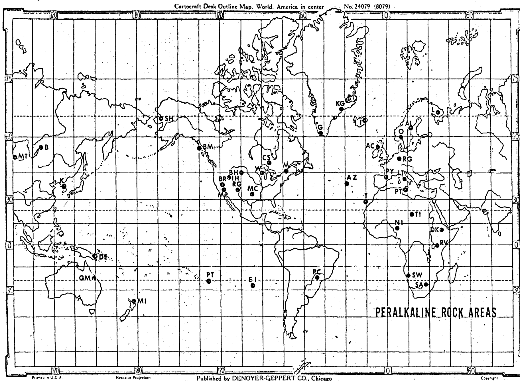
Fig. 5. World map showing locations of alkaline rock areas within which peralkaline intrusive bodies of significant size may occur. Legend: Refer to following page.
