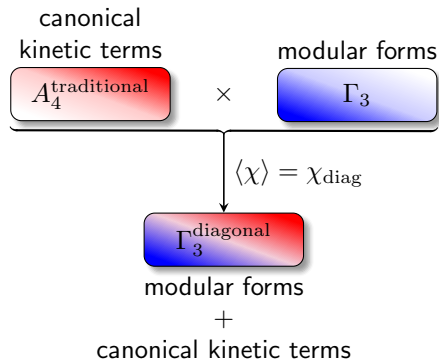
Figure 1: Diagonal breaking of traditional and modular flavor symmetries.
