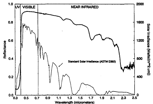
Fig. 1. Spectral reflectance of a high quality acrylic white coating (2 coats on a steel substrate). Also shown is the standard solar irradiance used as a weighting function for computing the overall solar reflectance (scale to right).
