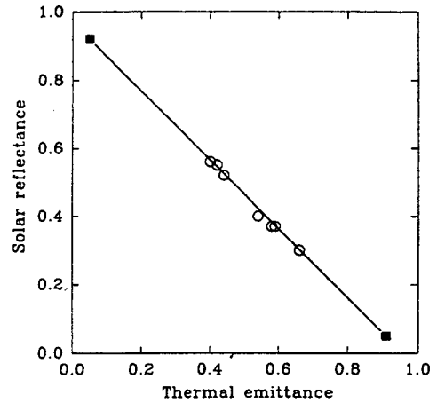
Fig. 5. Correlation between the solar reflectance and thermal emittance of aluminum roof coatings. End points are based on estimated values for bare aluminum and asphalt.
