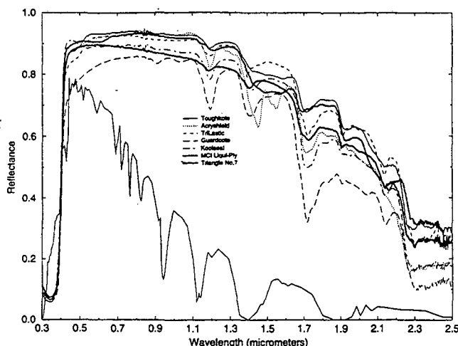
Fig. 2. Spectral reflectance of seven white roof coatings. Also, see Table 1.
