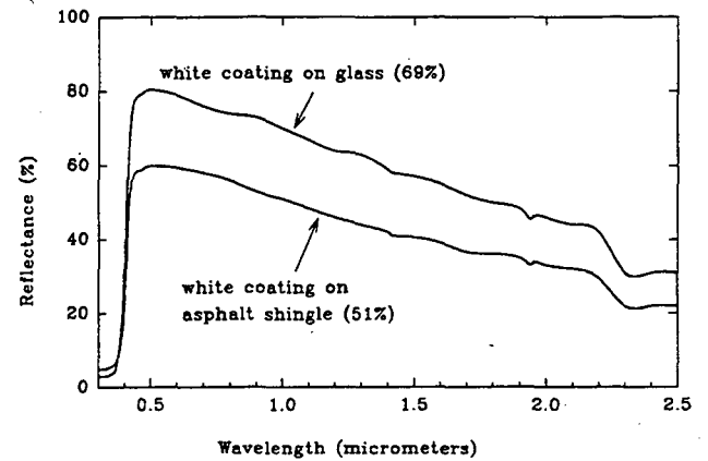
Fig. 7. Spectral reflectance of the same white coating applied to a smooth glass substrate, and on a rough asphalt shingle. The asphalt shingle is covered with granules, each about 1 mm in diameter.
