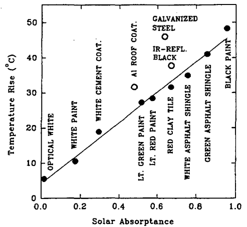
Fig. 11. Temperature rise above air temperature for twelve samples exposed to full sunlight on an insulated substrate. The filled circles are samples with emittances of about 0.9, and the open circles are samples with lower infrared emittances. The straight line is a fit to the data through the filled circles. Samples are described in the text.
