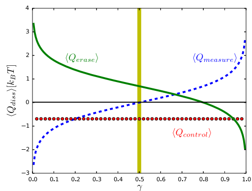
FIG. 3. Beyond Landauer's principle: Thermodynamic costs (energy dissipation Q_{\text{diss}} ) for measurement, control, and erasure in Szilard's information engine as a function of \gamma (demon partition) with SUS barrier at \delta = 1/2 . Landauer's principle applies only at \gamma = 1/2 (vertical yellow band at the middle): Measurements are thermodynamically free, but erasure costs because heat is dissipated as a result of demon resetting. Costs exactly flip at \gamma = 4/5 , though.
