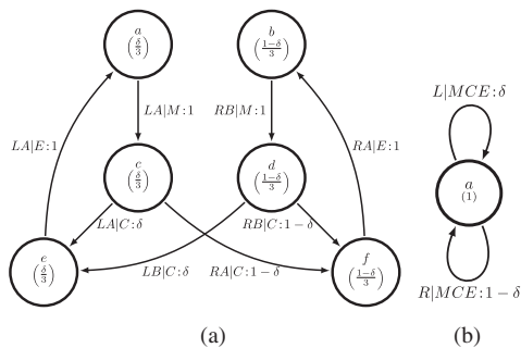
FIG. 2. \epsilon -Transducers for the symbolic dynamics of the Szilard information engine from the Markov partition of its joint state space. (a) The \epsilon -transducer for \mathcal{T}_{\text{Szilard}} that reads in the periodic control signal for measure ( M ), control ( C ), and erase ( E ). (b) \mathcal{T}_{\text{Szilard}} single-state \epsilon -transducer: Memoryless over the full measure-control-erase protocol. Transitions \beta|\alpha: p denote reading protocol symbol \alpha , taking the transition with probability p , and emitting symbol \beta . Asymptotic state probabilities are given in parentheses underneath state names.
