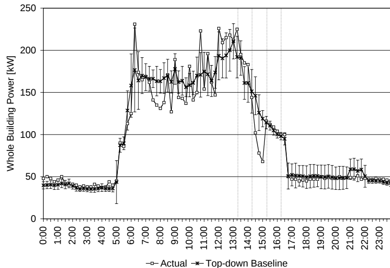
Figure VII-29. Roche – Building FS, Whole Building Power and Baseline
