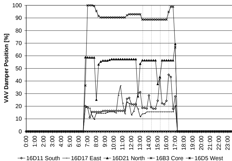
Figure VII-26. GSA – South 16th Floor VAV Damper Position
