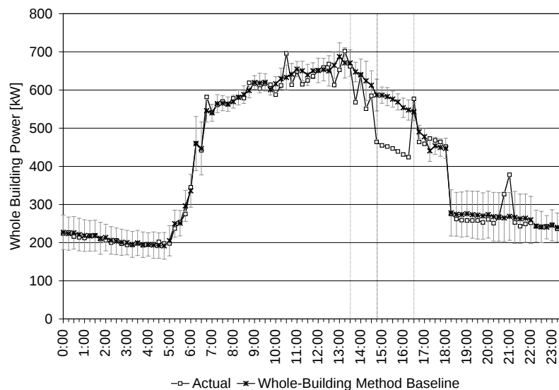
Figure VII-5. Roche – Whole Building Power and Baseline (1st Day)
