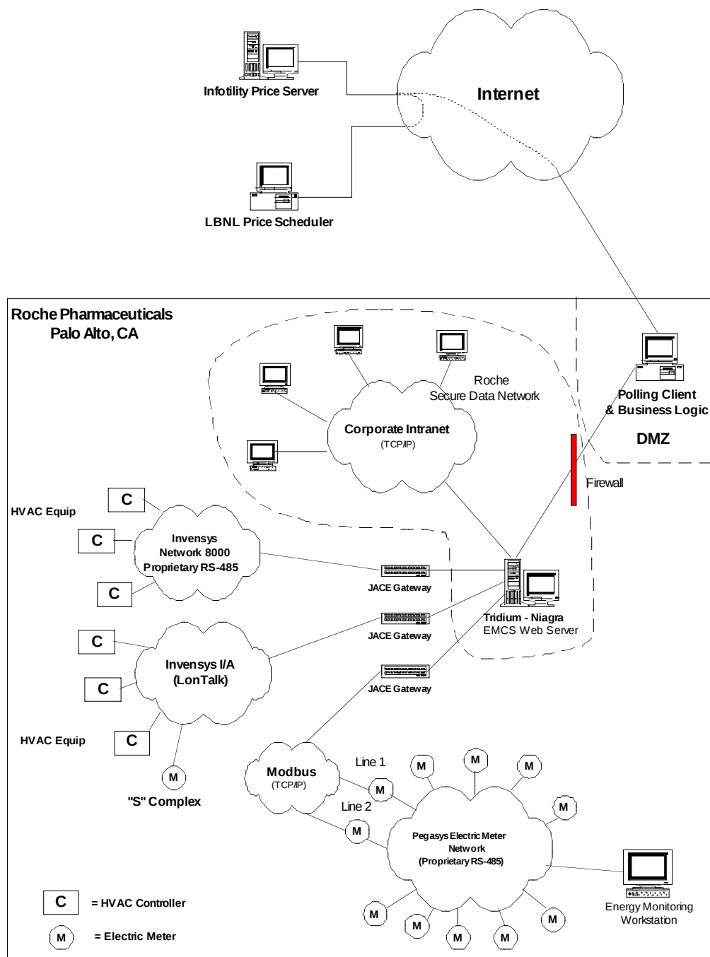
Figure 3-15. Roche – System Architecture
