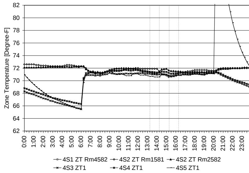
Figure VII-35. UCSB – Library IV, Zone Temperatures
