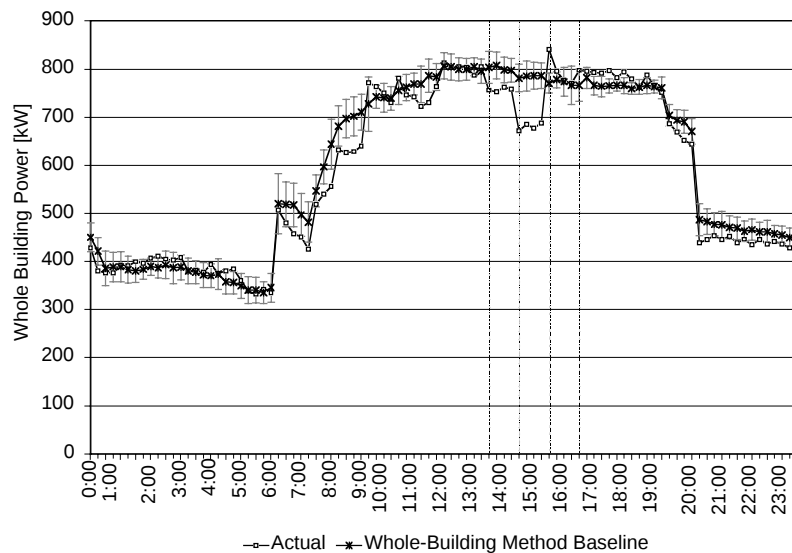
Figure 4-33. UCSB – Whole Building Power and Baseline (Whole-Building Method)
