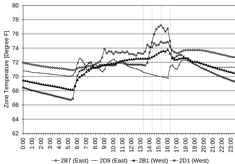
Figure VII-20. GSA – South Tower 2nd Floor Zone Temperature
