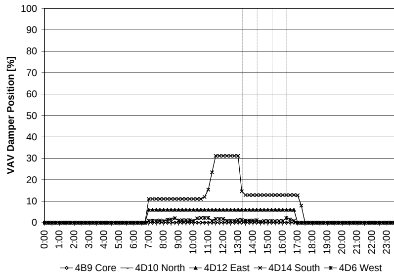
Figure VII-25. GSA – South 4th Floor VAV Damper Position
