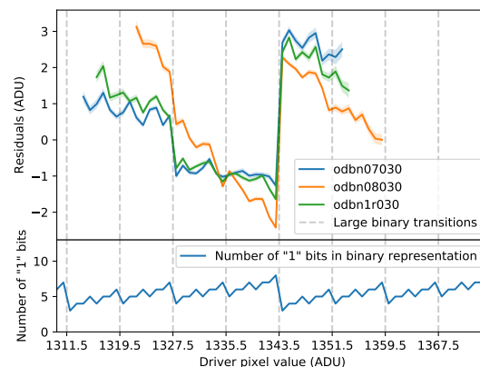
(d) STIS (HST), 1 pixel after the driver pixel. The median measurement uncertainty for the residuals is 0.077 ADU.
