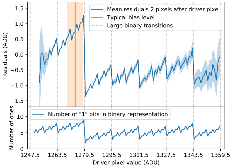
Figure 2. Example of the binary offset effect on the SNIFS blue channel right amplifier. See text for details on how this plot was produced. Top panel: mean residuals as a function of the raw driver pixel value read out 2 pixels earlier along with an uncertainty band. Bottom panel: number of "1" bits in the binary representation of the driver pixel value. We label transitions where more than 5 bits flip with a vertical dashed line. All of the features in the bottom panel, including the large transitions, are visible in the residual data. The mean background level and one standard deviation of read noise are illustrated with a vertical orange line and surrounding band.
