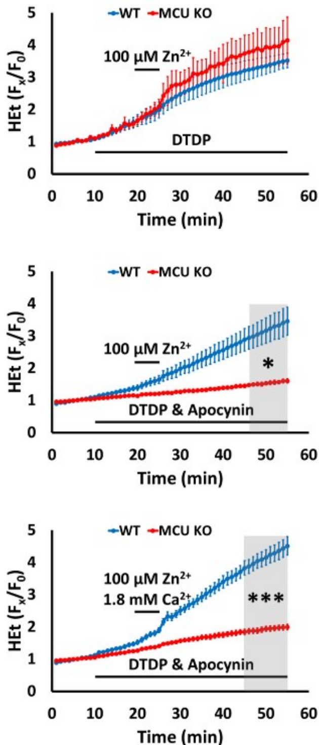
Figure 2. Zn^{2+} -triggered mitochondrial—but not cytosolic—ROS production is attenuated in MCU KO neurons. WT (blue) and MCU KO (red) cultured neurons loaded with superoxide preferring ROS indicator Hydroethidine (HET) in either 0 mM Ca^{2+} (top and middle) or 1.8 mM Ca^{2+} (bottom) HSS were exposed to 100 \mu M Zn^{2+} + high K^+ , with DTDP (60 \mu M ) and apocynin (500 \mu M ) added as indicated. Traces display mean \pm SEM F_x/F_0 values for HET \Delta F and represent \geq 8 experiments consisting of \geq 160 neurons. Grey bars indicate time points of comparison (* indicates p < 0.05 , *** indicates p < 0.001 , by two-tailed t-test). Despite the similar total ROS generation (top), note that Zn^{2+} -triggered ROS rise specifically from
