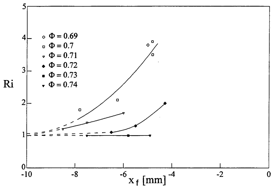
Figure 14 : Richardson number, Ri , determined for cases of Table I according to Equation (4).
