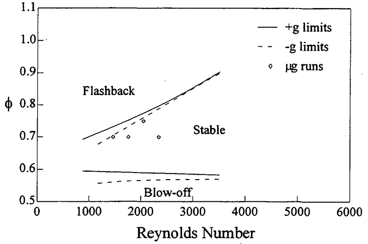
Figure 2 Blow-off and Flash-back limits for (a) laminar v-flames and (b) turbulent v-flames
