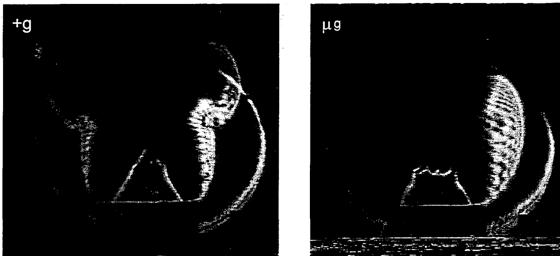
Figure 5 : Schlieren records of a laminar conical flame stabilized showing changes in flame shape from normal gravity (+g) to microgravity ( \mu g ).
