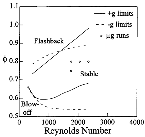
Figure 2 Blow-off and Flash-back limits for (a) laminar v-flames and (b) turbulent v-flames
