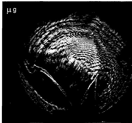
Figure 3 : Schlieren records of a \mu\text{g} laminar V-flame showing changes in flame shape from normal gravity (+g) and microgravity ( \mu\text{g} ).
