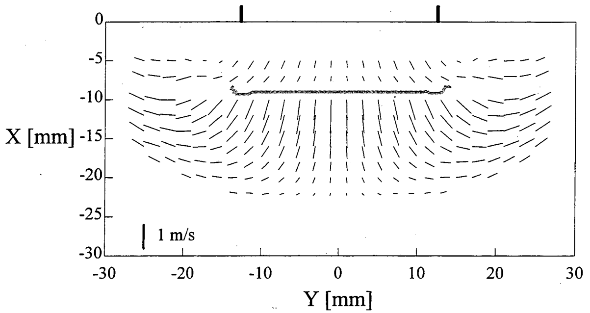
Figure 9 : Velocity vector measure in a buoyancy stabilized flame of Q = 0.19 l/s, \phi = 0.735
