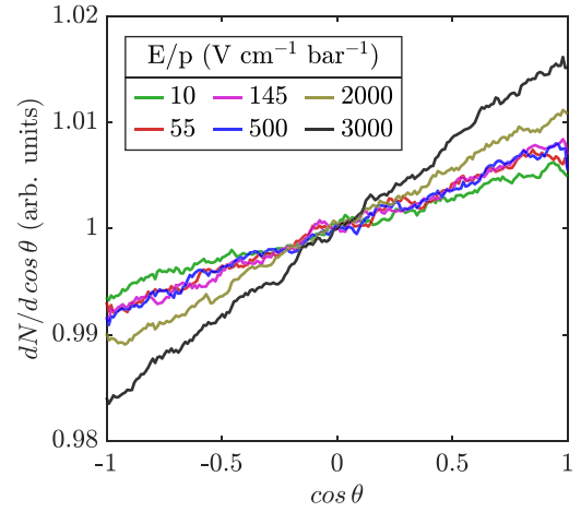
FIG. 1. Angular distributions ( dP/d \cos \theta ) obtained for the angle between the electron momentum vector and the direction of the electric field, prior to each collision, obtained with the transport code pyboltz . For clarity, data are smoothed by a moving average.
