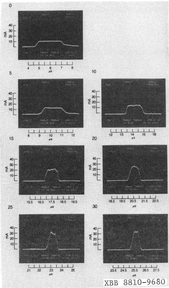
Figure 1. Current waveforms at each diagnostic gap through the linac under the gentle schedule.
