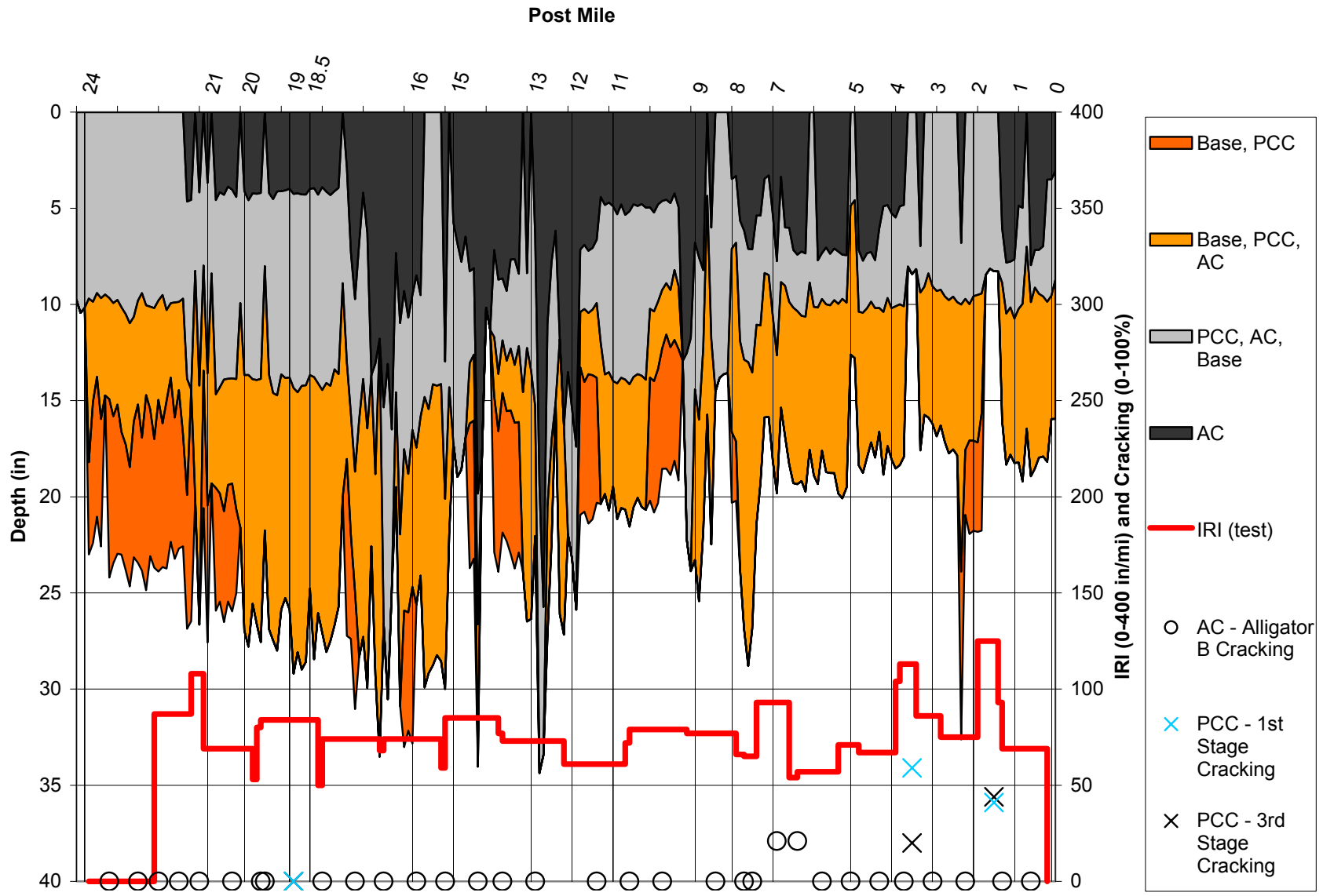
Figure C1. GPR cross section with selected PCS data – Sacramento SR-99 SB (outside lane), CAL099.
