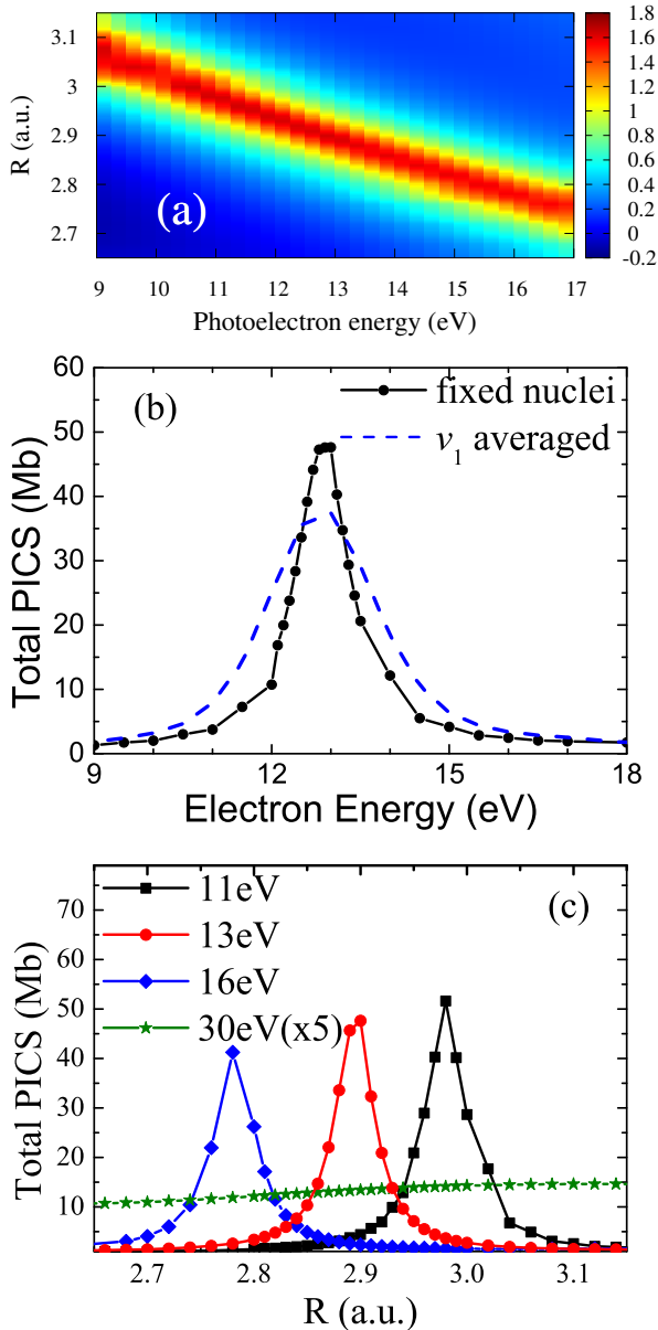
FIG. 3. (Color online) (a) Total PICS (in logarithmic scale) vs photoelectron energy and S-F separation. (b) Total PICS vs photoelectron energy for SF 6 at equilibrium. Results after averaging over \nu_1 = 0 is shown as the dashed line. (c) Total PICS vs S-F internuclear distance R for a few photoelectron energies. The PICS at 30 eV has been multiplied by a factor of 5.
