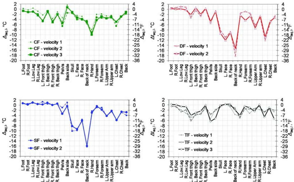
Figure 7. Change in manikin-based equivalent temperature ( \Delta t_{eq,i} ) on each body part from the reference condition (room temperature equal to 25^{\circ}\text{C} and no devices used for air movement) for the ceiling fan (top left), desk fan (top right), standing fan (bottom left), and tower fan (bottom right). Step-change control of the fan velocity is possible. The \Delta t_{eq,i} was calculated for the different speed levels reported in Table 1.
