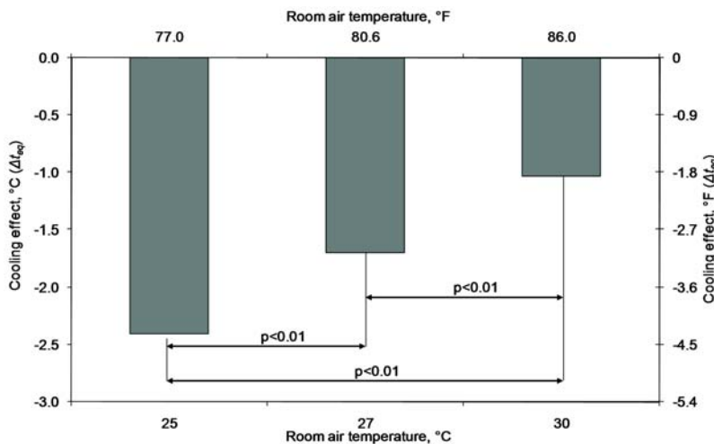
Figure 6. Averaged (over the type of cooling fan and speed level) cooling effect for three room air temperatures.
