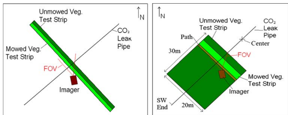
Fig. 2 Layout of the mown and unmown vegetation test segments and the multispectral imager during the 2007 ( left ) and 2008 ( right ) CO 2 release experiments. The 55° full-angle imager field of view ( FOV ) is indicated by the red lines
