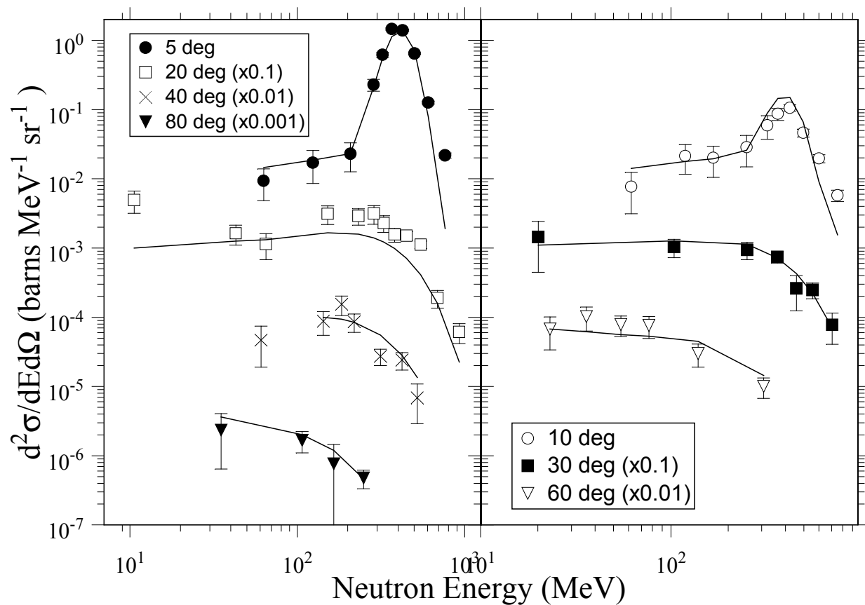
Fig. 9. Double-differential spectra from 400 MeV/nucleon Kr interacting in a \text{CH}_2 target. The spectra at each laboratory angle are offset by the indicated factors of 10. The lines come from a moving-source fit described in the text.
