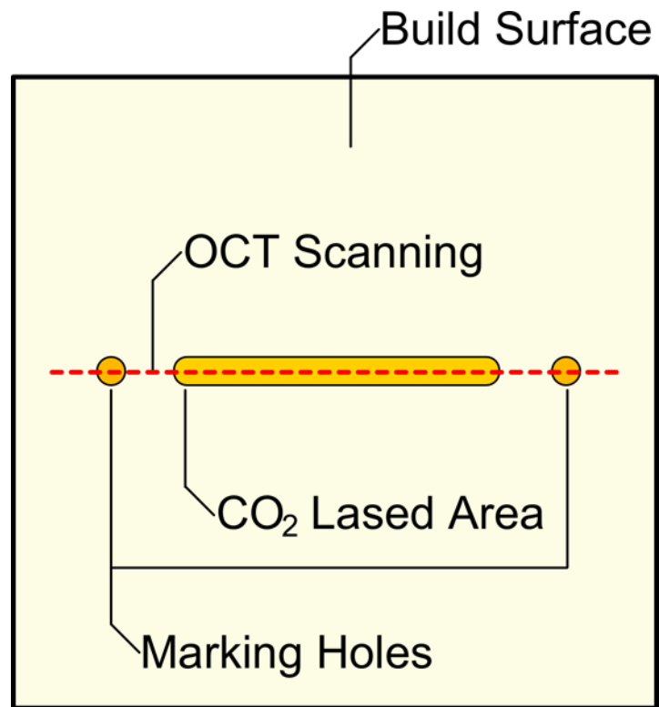
Fig. 3. En-face view of the build surface. The orange sections indicate areas of nylon sintering; the red dotted line is the OCT beam path.
