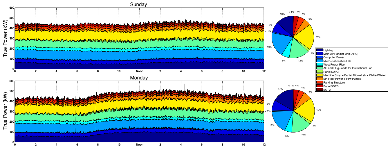
Figure 10. A detailed breakdown of electrical usage inside the Electrical Engineering building over two days. Data is pushed to a client database by a sMAP gateway connected to three Dent circuit meters, each with six channels. Power is used primarily by lighting, HVAC, and a micro-fabrication lab, as expected. Interestingly, the total power consumed on Sunday is 440kW while on Monday is 462kW, an increase of less than 5% between a weekend and a weekday, indicative of an inefficient building. The difference between day and night is small as well. The only load with an obvious spike in power is lighting at around 7am on Monday, whereas most loads stay the same throughout the day and night.
