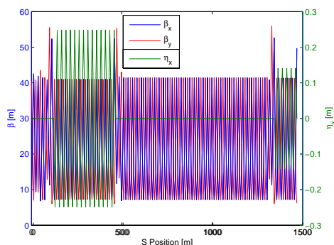
Figure 2: Twiss parameters of two-stage bunch compressor.
