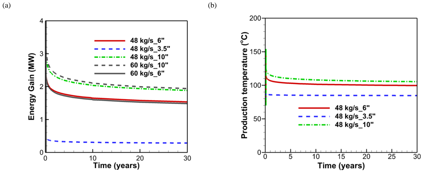
Figure 6: Simulation results of the effect of pipe diameter on energy gain in the closed loop. (a) High flow rates in large-diameter pipes favor heat transfer to the pipe. (b) At fixed flow rate, larger temperatures develop in larger-diameter pipes in the closed loop.
