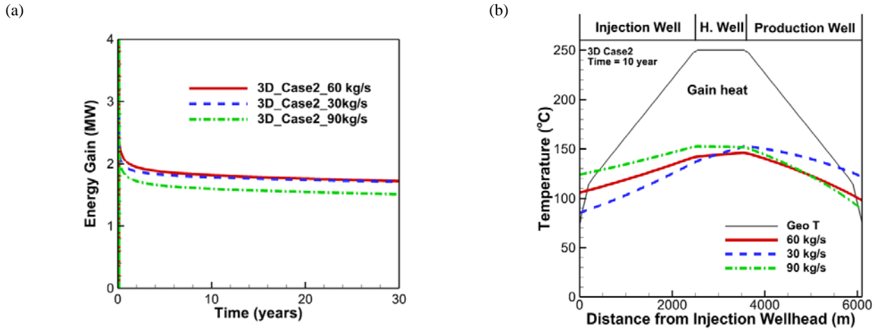
Figure 5: Simulation results of the effect of different CO 2 flow rates on energy gain in the closed loop for the low-permeability (Case 2) reservoir. (a) Intermediate flow rate (60 kg/s) is better than 30 kg/s or 90 kg/s for energy recovery; (b) Only the low flow-rate case results in CO 2 temperature higher at outlet than at inlet of closed loop.
