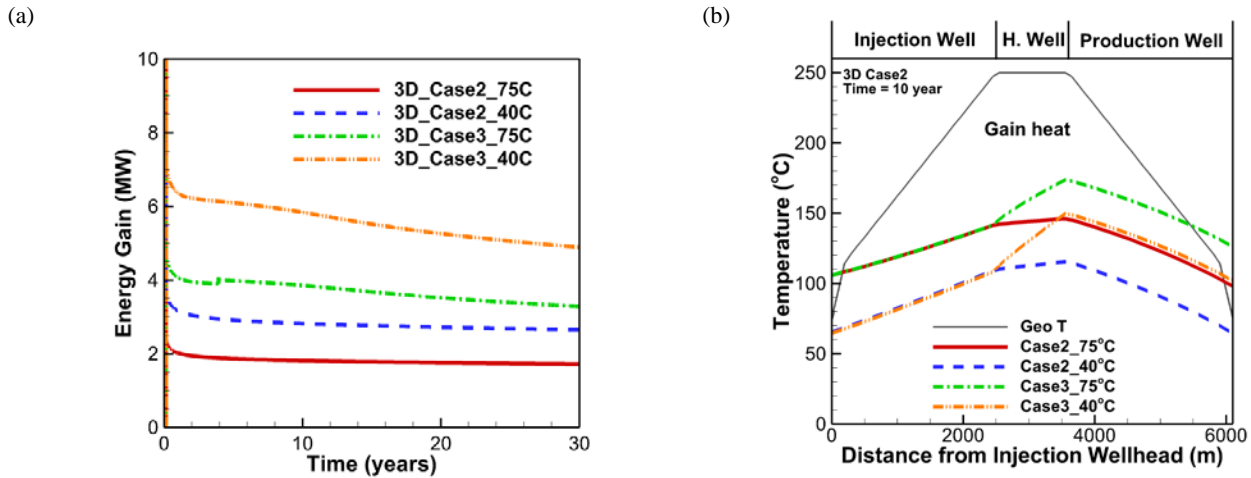
Figure 4: Simulation results of the effect of different inlet CO 2 temperatures on energy gain in the closed loop for the low-permeability (Case 2) and high-permeability (Case 3) reservoirs. (a) Low inlet temperature improves energy recovery; (b) Heating due to convection of heat from reservoir to CO 2 occurs for high-permeability (Case 3) reservoir.
