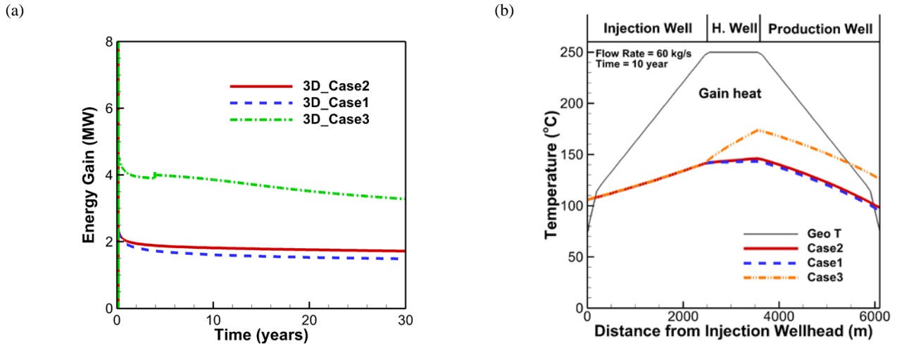
Figure 3: Simulation results of the effect of reservoir permeability on energy gain in the closed loop. (a) High-permeability in the reservoir favors convective heat transfer to the pipe. (b) The effects of convective heat transfer to the pipe are largest in the horizontal section of the closed loop.
