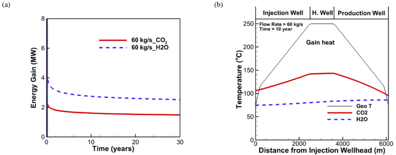
Figure 7: Simulation results for CO 2 and H 2 O as working fluids. (a) Water gains more energy through the loop at 60 kg/s than CO 2 . (b) Water temperature increases in each part of the closed loop whereas CO 2 temperature may decline due to decompression effects.
