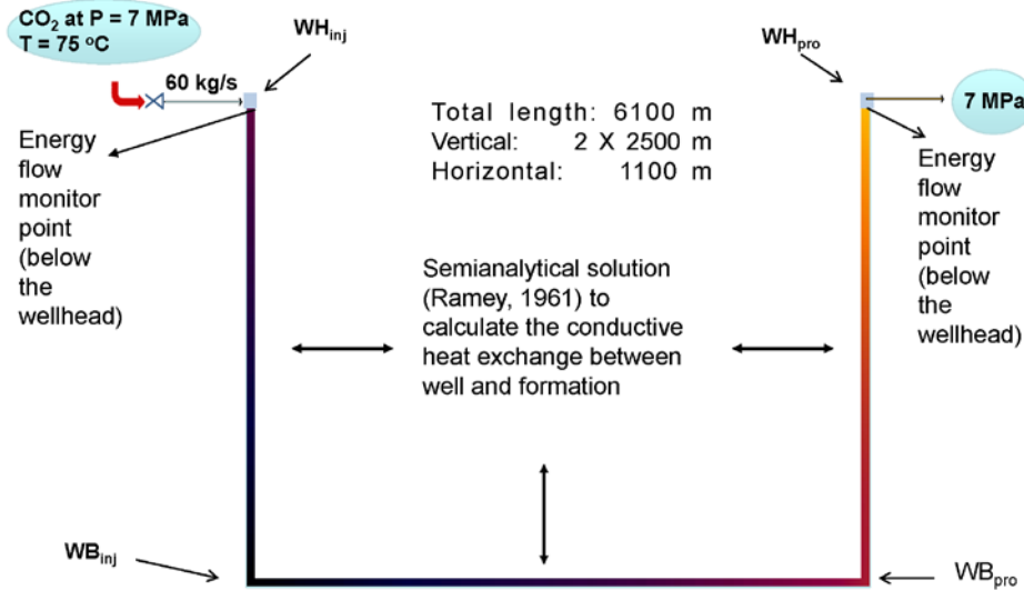
Figure 1: Sketch of closed loop geothermal energy system for CO 2 flowing from inlet (upper left-hand side) to outlet (upper right-hand side). WH inj = wellhead of injection leg; WB inj = wellbottom of injection leg; WB pro = wellbottom of production leg; WH pro = wellhead of production leg.
