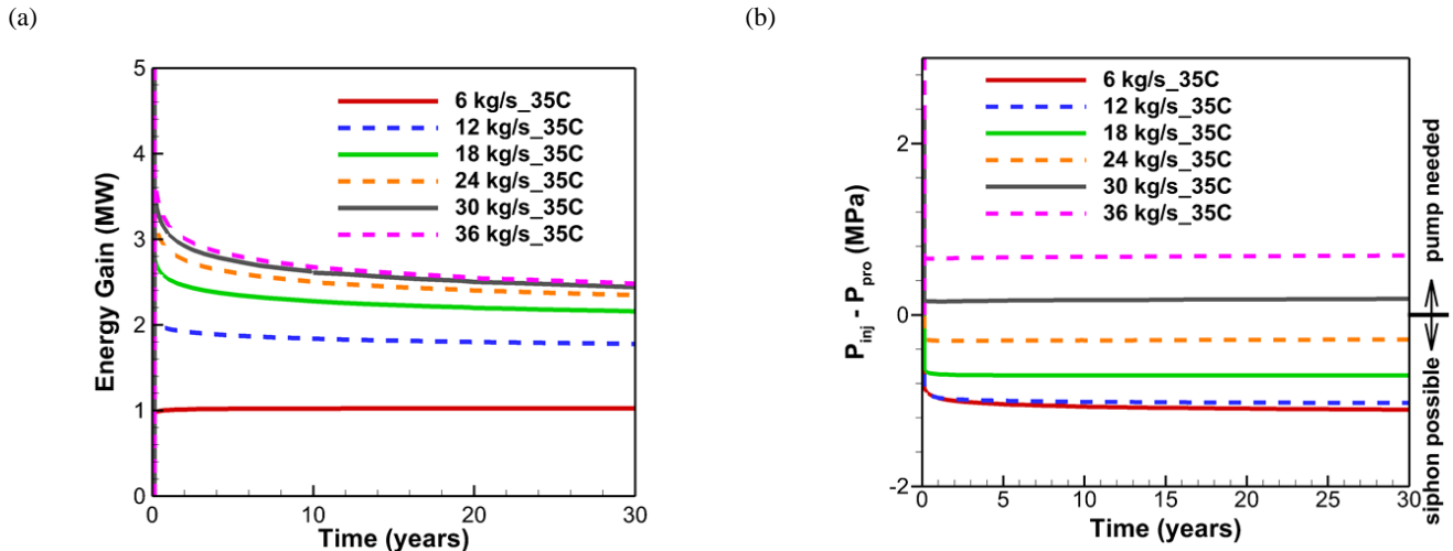
Figure 8: Simulation results for various CO 2 flow rates. (a) Energy gain correlates directly with flow rate at 35 °C inlet temperature. (b) The closed loop will operate without need for pump only at flow rates below about 25 kg/s.
