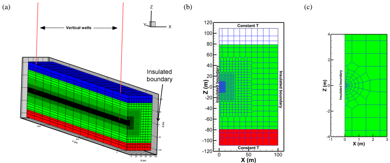
Figure 2: Discretization of the reservoir part of the closed-loop model showing (a) 3D domain (blue = overburden, red = underburden, and green = reservoir region) including the vertical legs (red lines) of the closed-loop well, (b) cross section of the horizontal well region, and (c) closeup of the well region.
