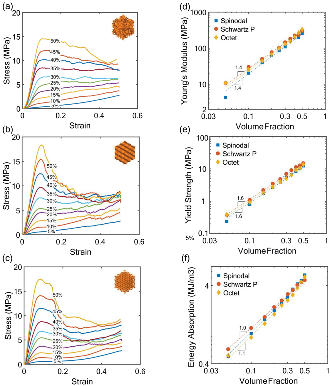
Fig 5. (a-c) Stress-strain curves of IPCs with different reinforcement topologies at various volume fractions compressed to 50% strain. Notice that spinodal shell IPCs don't exhibit catastrophic load drops at high volume fractions of reinforcement. (d- f) Comparison of mechanical properties of IPCs at different reinforcement volume fractions: (d) Young's modulus; (e) Yield strength; (f) Energy absorption. Mechanical properties of spinodal IPC at 5% were excluded from the scaling as the thickness of the reinforcement shell is close to the resolution of the 3D printer and is susceptible to manufacturing defects.
