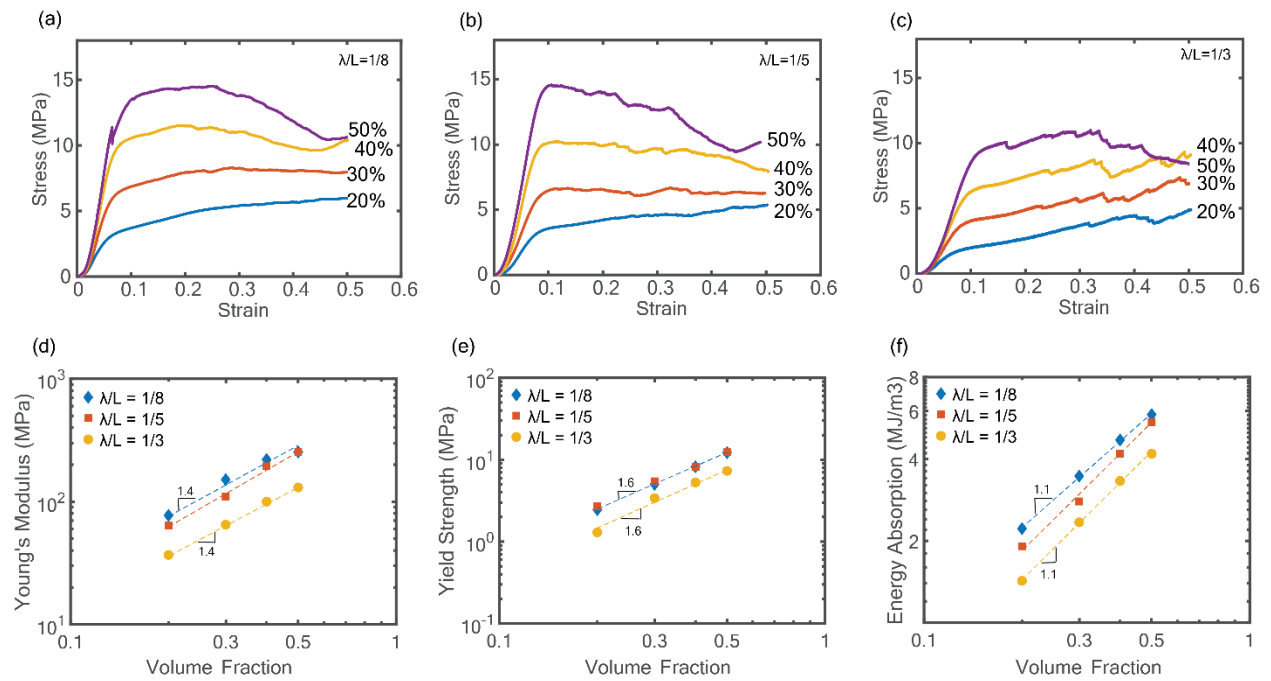
Fig. D. 3. Mechanical properties of spinodal shell IPCs with different curvature/surface area. Stress-strain curves for (a) \lambda/L = 1/8 ; (b) \lambda/L = 1/5 ; (c) \lambda/L = 1/3 . (d) Young's modulus. (e) Yield strength. (f) Energy absorption.
