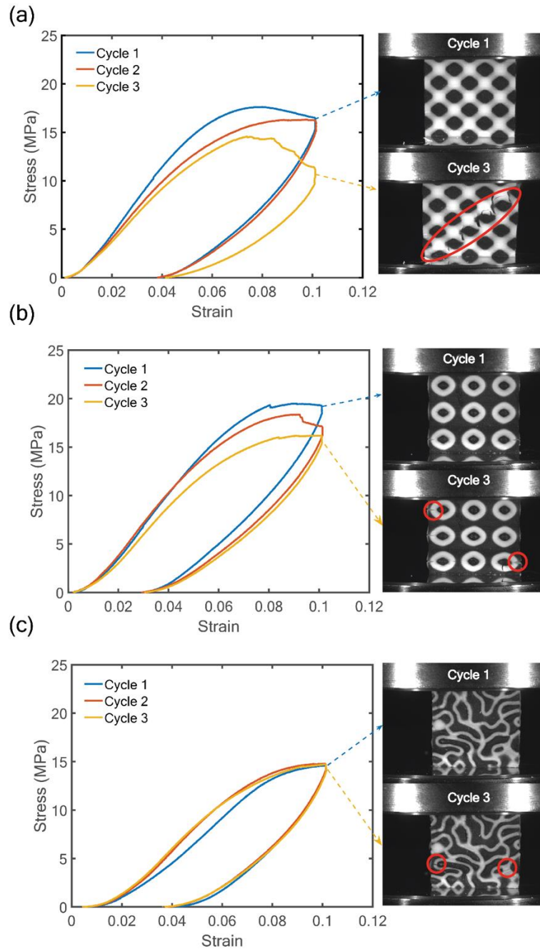
Fig 7. Cyclic compression experiments on IPCs with different reinforcement topologies, at 50% volume fraction of reinforcement. All samples have been compressed to 10% strain for 3 cycles. (a) Octet lattice composite. (b) Schwartz P shell composite. (c) Spinodal shell composite. All three topologies show increasingly visible fractures in the reinforcement phase as cycling loading progresses. Both periodic IPCs show decreasing load bearing capacity as a result, while the stress-strain curve of the spinodal shell composite is largely unaffected.
