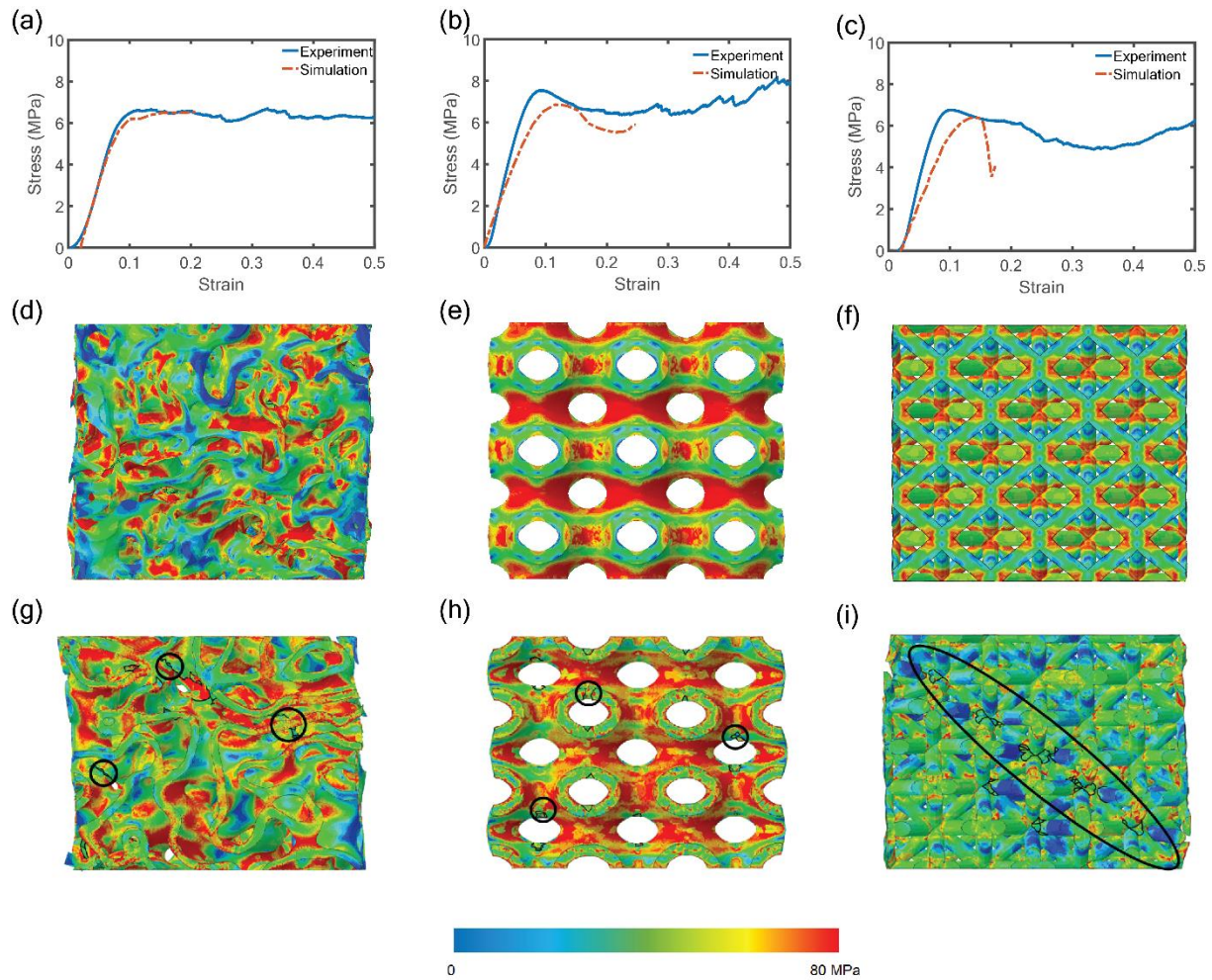
Fig 8. Comparison between experiment and simulation results. (a, b, c) Stress strain curve comparison between experiment and simulations, for IPCs at 30% volume fraction of reinforcement: (a) spinodal shell IPC; (b) Schwartz P shell IPC; (c) octet lattice IPC. (d, e, f) von Mises stress map of the reinforcement phase, extracted from the composite at 10% strain: (d) spinodal shell reinforcement; (e) Schwartz P shell reinforcement; (f) octet lattice reinforcement. (g, h, i) von Mises stress map of the reinforcement phase at the half-way cross section, extracted from the composite at 15% strain: (g) spinodal shell reinforcement; (h) Schwartz P shell reinforcement; (i) octet lattice reinforcement. Cracks are highlighted in black.
