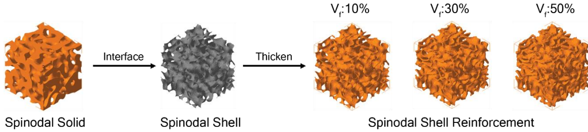
Fig 1. Schematic of approach for numerically generating the spinodal shell reinforcement phase for IPCs.
