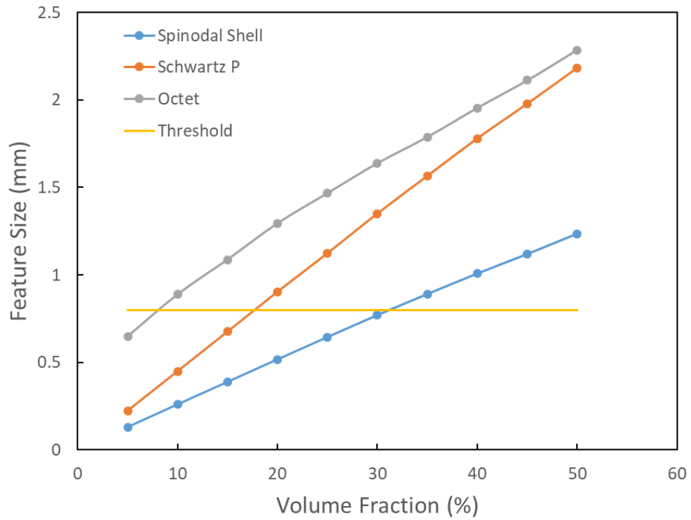
Fig. B.2. Feature size of the reinforcing phase as a function of the volume fraction of reinforcement, for different topologies. The yellow horizontal line represents the threshold below which size effects are expected.
