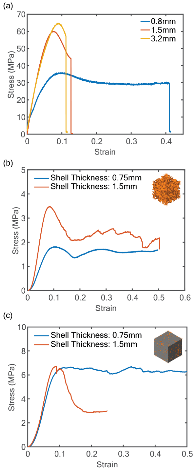
Fig. B.1. (a) Stress-strain curves of tensile samples with different thickness; (b) Compressive stress-strain curves of spinodal shell cellular (reinforcement only) sample at 30% volume fraction of reinforcement, for different shell thicknesses; (c) Compressive stress-strain curves of spinodal shell IPC at 30% volume fraction of reinforcement, for different shell thicknesses.
