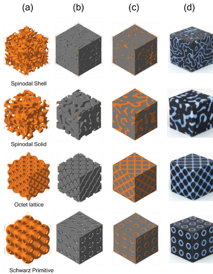
Fig 2. (a) Reinforcement phase, (b) matrix phase, (c) assembled interpenetrating phase composite and (d) 3D printed composite sample for spinodal shell, spinodal solid, octet lattice and Schwarz P shell IPCs.
