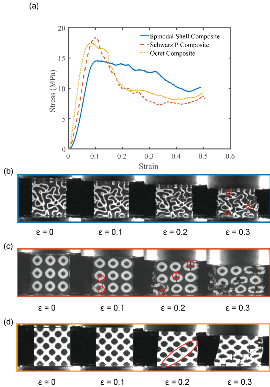
Fig 6. Deformation response of IPCs with different reinforcement topologies at 50% volume fractions, compressed to 50% strain. (a) Stress-strain curve. (b) Spinodal shell composites. (c) Schwarz P shell composites. (d) Octet lattice composites. Notice that octet and Schwarz P IPCs at high volume fraction of reinforcement experience more localized catastrophic failures than spinodal shell IPCs.
