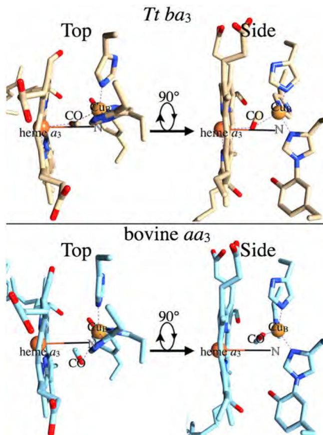
Fig. 8. Top panel: The Tt ba3 Cu B -CO transient photoproduct (PDB 3QJR, 49). Lower panel: The bovine Cu B -CO transient photoproduct (PDB 3AG2, 55). In both panels, the left figure (Top) is viewed from the positive side of membrane, while the right figure (Side) is viewed from the ligand entrance channel. The “Side” view is generated from the “Top” by a left-handed 90° rotation about the horizontal axis.
