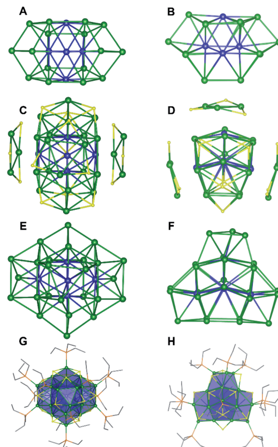
Fig. 1 Solid-state structure of [Ni 30 S 16 (PET 3 ) 11 ] · Et 2 O ( 1 · Et 2 O) from two different orientations. (A and B) Ni 30 S 16 core. (C and D) The three [ cyclo -{Ni(μ-S)} 3 ] units attached to the Ni 21 S 7 core. (E and F) Ni-only structure of 1 . (G and H) Full molecular structure. Color scheme: Ni shell , green; Ni core , blue; S, yellow; P, orange; C, grey. Carbon atoms are shown in wireframe. Diethyl ether solvate molecule and hydrogen atoms were omitted for clarity.
