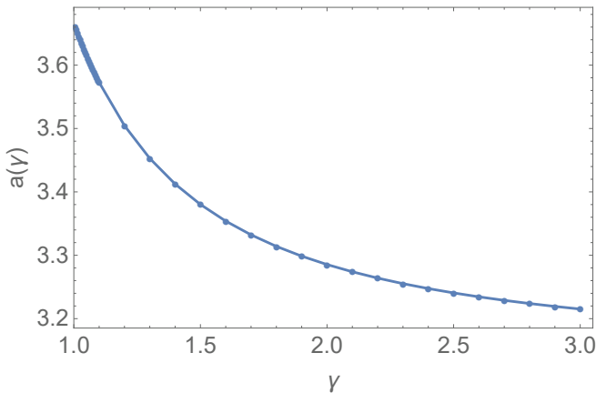
FIG. 3. Exponent a in L/L_0 = \gamma^{a(\gamma)} for the Luttinger liquid model. The dependence on \gamma is stronger than in the generalized noninteracting model. Lines are given by linear interpolation between adjacent data points, and error bars are omitted for clarity.
