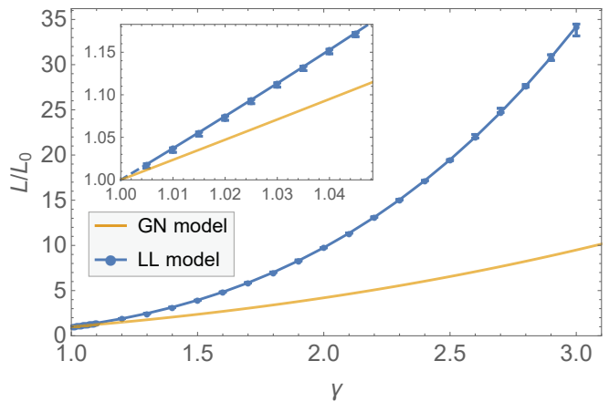
FIG. 1. (Color online) Lorenz number, L , as calculated in the generalized noninteracting (GN) and Luttinger liquid (LL) models. The Lorenz number is plotted as a function of the interaction strength \gamma in units of L_0 , the value expected from the Wiedemann-Franz law. For both models, we find that L = L_0 in the noninteracting case \gamma = 1 . Electron-electron interactions ( \gamma > 1 ) lead to a violation of the Wiedemann-Franz law; the violation is stronger in the LL model than in the GN model. The Lorenz number is evaluated at discrete points in the LL model; error bars indicate the precision of numerical results as described in the text. Lines connecting the data points for the LL model show linear interpolation between adjacent points, and the dashed line below \gamma = 1.005 in the inset shows extrapolation to \gamma = 1 .
