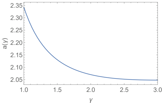
FIG. 2. The Lorenz number scales as L/L_0 = \gamma^{a(\gamma)} . For the generalized noninteracting model we find 2 < a(\gamma) < 2.35 for all \gamma , with L \approx L_0 \gamma^2 for large \gamma .
