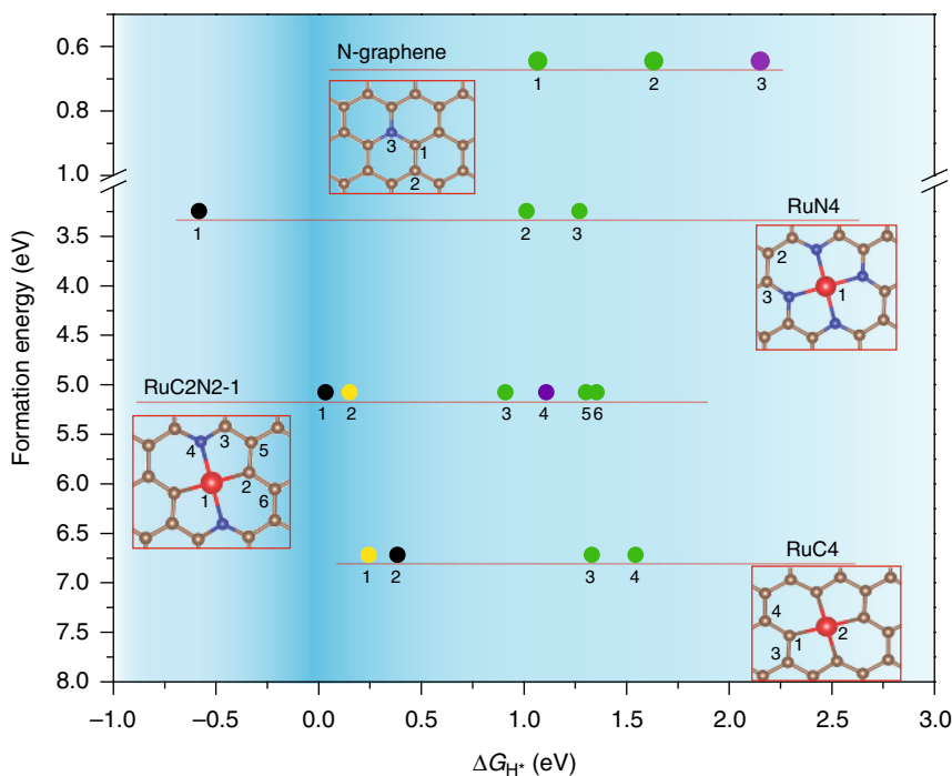
Fig. 5 Energy diagram of different \text{Ru}_x\text{N}_y structures from first principles calculations. The x axis is reaction free energy of hydrogen binding, where the negative values indicate strong binding while positive values indicate weak binding. The dark blue range indicates the candidate active sites with the best activity. The y Axis is formation energy of each configuration, where a more positive value signifies a structure that is more difficult to form. The colors denote candidate active sites: H binds to a ruthenium atom along the perpendicular direction to the plane (black), a carbon atom next to the ruthenium (yellow), a carbon atom next to nitrogen (green), or a carbon atom far away from ruthenium and nitrogen atoms (purple). The note records the data point from a certain structure, number records the possible active site. The version with complete \text{Ru}_x\text{N}_y configurations can be found in Supplementary Figure 14 and the structures can be found in Supplementary Figure 15
