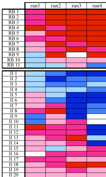
Figure 2: RB and II model fits for RB (top) and II subjects (bottom). Fit values were separated into thirds with darker hues (i.e. from pink to red for RB fits) indicating better fit. RB fits are in warm and II in cool colors. The darkest hues were included in the fMRI analysis. White blocks indicate data loss due to subject movement.
