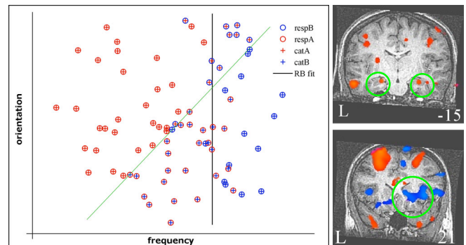
Figure 5: One II subject (#18, run 4) run that was best fit with the RB model (left) and the corresponding contrast of correct vs. incorrect trial activity (right). Plus signs indicate the category membership of the stimuli whereas the circles show the pattern of subject responses. Instances where colors agree indicate correct responses and all others are incorrect. The green line indicates the optimal decision boundary and the black line the best fitting account of the data according to the RB model.
