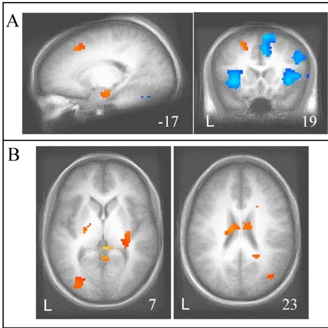
Figure 4: Correct (red) vs. incorrect (blue) trials for (A) best RB model fit runs and (B) best II model fit runs. All images were thresholded at T > 4 , \text{cluster} > 350 \text{mm}^3 . When fMRI data was grouped according to model-fit value, activity was detected in areas consistent with the COVIS theory of category learning.
