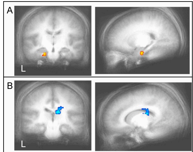
Figure 3: RB vs. II, correct vs. incorrect trials in the (A) MTL and (B) Caudate ROIs. In the left anterior MTL, successful RB categorization activity was greater than that of the II group. In contrast, II successful categorization was greater in the right posterior body of the caudate than RB categorization activity.
