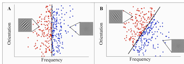
Figure 1: (A) RB and (B) II category learning tasks. Each point represents a distinct Gabor patch (sine-wave) stimulus defined by orientation and frequency (thickness of lines). In both stimulus sets, there are 2 categories (red and blue points). RB categories are defined by a vertical boundary (only frequency is relevant) and II categories by a diagonal boundary (both dimensions are relevant). In both stimulus sets there are examples of a stimulus from each category.
