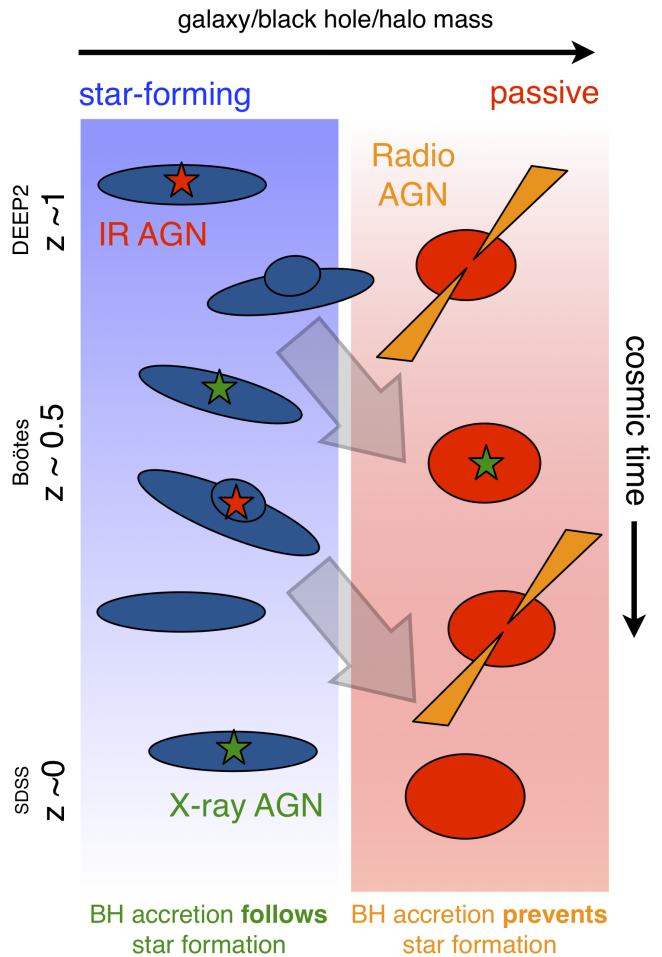
FIG. 7.— Schematic diagram of the evolution of AGN host-galaxies throughout the last 9 Gyrs of Cosmic time. From the results presented here, we find that galaxy evolution follows an apparently similar path at all redshifts. All galaxies appear to begin as star-forming blue-cloud systems and end as passive red-sequence sources, once their dark matter halos have grown sufficiently. However, we show that those galaxies hosting IR, X-ray and/or radio AGN appear to follow a similar evolutionary path: radiatively-efficient rapid BH growth (IR/X-ray AGN) appears to be linked with those galaxies with large supplies of cool gas, while mechanically dominated (radio) accretion is associated with passive galaxies, which may also be responsible for preventing late star-formation.
