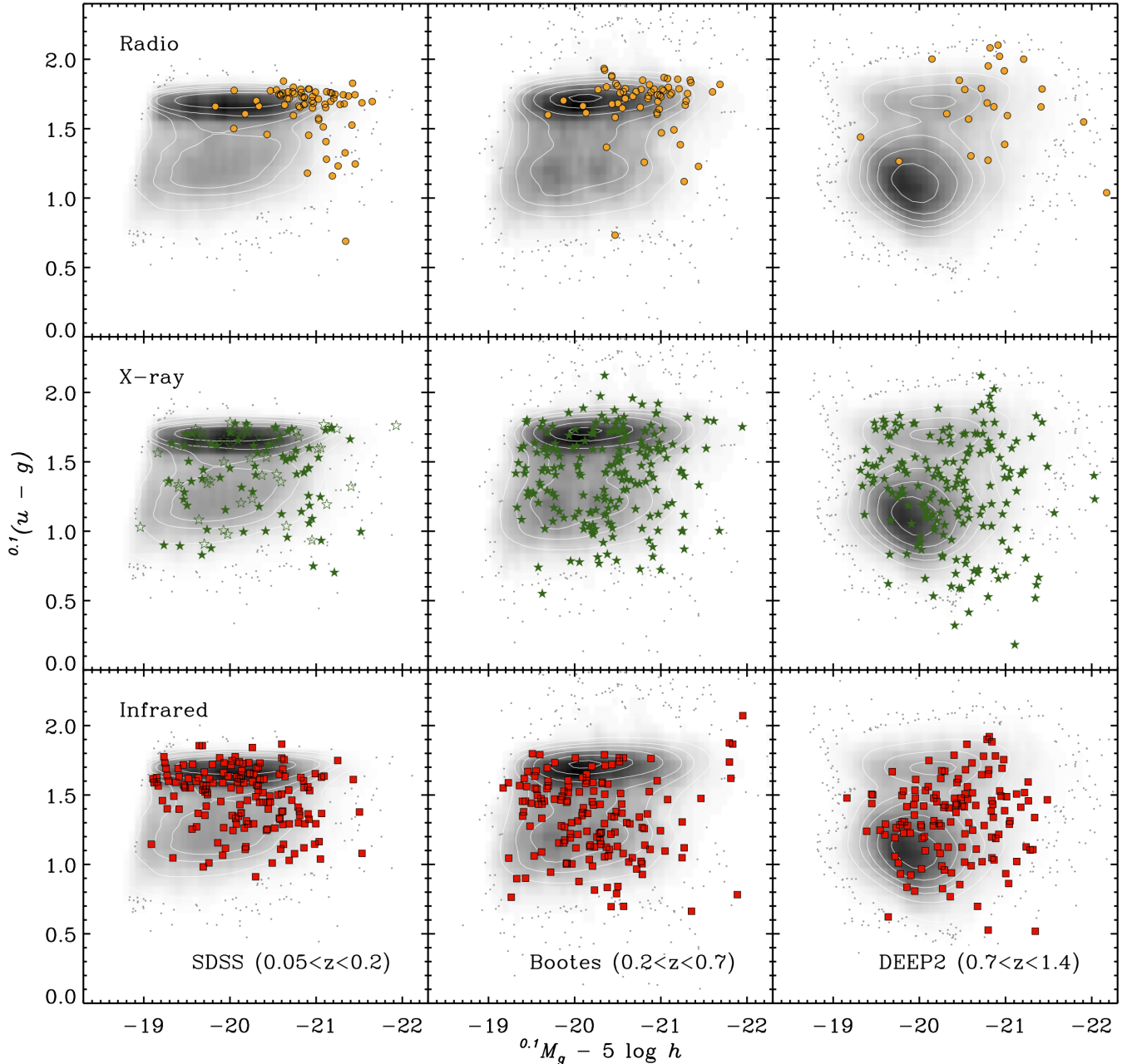
FIG. 5.— Rest frame optical color–magnitude distributions of AGN hosting galaxies at z < 0.2 (SDSS; left column), 0.2 < z < 0.7 (Boötes; center column) and 0.7 < z < 1.4 (DEEP2; right column). Photometry for the galaxy samples have been K -corrected and converted to equivalent SDSS u and g filters at z = 0.1 , and absolute g -band magnitudes are corrected for passive evolution (e.g., Blanton et al. 2003; 2007). The color–magnitude diagrams for the selection-matched galaxy populations, in each redshift range, are shown with grayscale contours. Overlaid on the optical color–magnitude diagrams are radio ( P_{1.4\text{GHz}} \gtrsim 10^{24} \text{W Hz}^{-1} ), X-ray ( L_X \gtrsim 10^{42} \text{erg s}^{-1} ) and IR-selected AGN which are shown with filled orange dots, green stars and red squares, respectively. Low-redshift ( z < 0.2 ) X-ray AGN identified in the SDSS (with L_X \sim 10^{41}–10^{42} \text{erg s}^{-1} ) are shown with open green stars. From Markov-Chain Monte Carlo 2-dimensional Kolmogorov-Smirnov testing, we find that in each redshift regime, radio AGN are almost exclusively hosted in passive red galaxies with little evidence for evolution in their host-galaxy color–magnitude distributions. Furthermore, we find that at all redshifts X-ray AGN are spread throughout the color–magnitude diagram, with similar distributions at all redshifts, while IR AGN may show marginal evidence for evolution between 0.7 < z < 1.4 and 0.2 < z < 0.7 .
