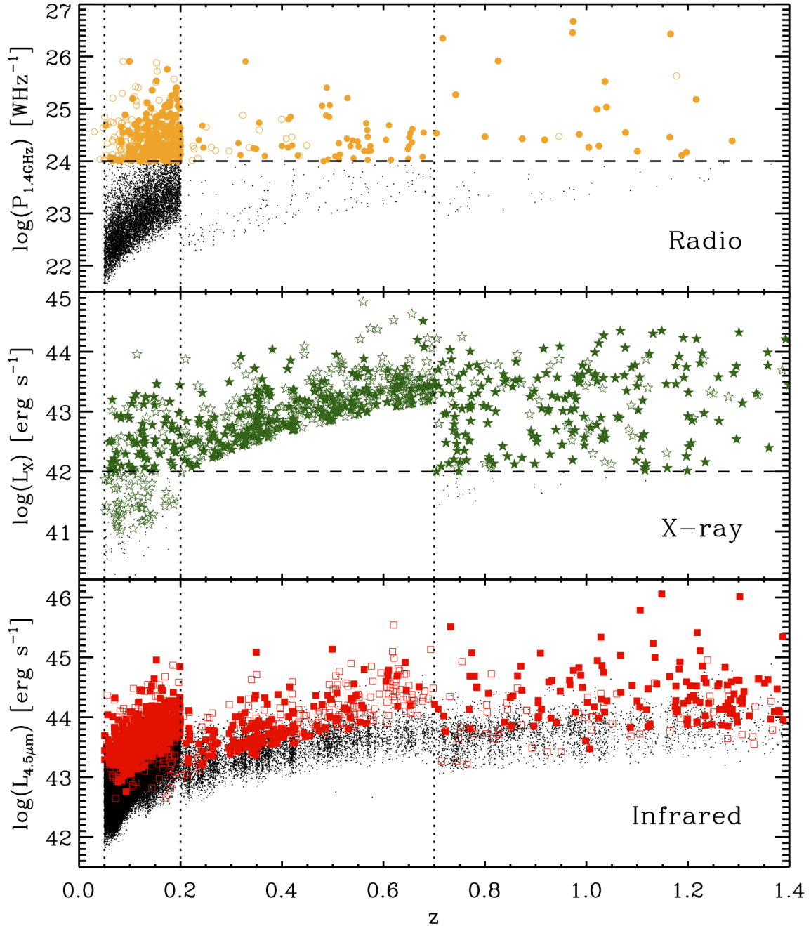
FIG. 4.— Luminosity distributions of galaxies (dots) and radio, X-ray and IR AGN (filled circle; star; squares, respectively) in the survey samples. Radio AGN are selected at the threshold of P_{1.4\text{GHz}} > 10^{24} \text{ W Hz}^{-1} , and X-ray AGN with L_X > 10^{42} \text{ erg s}^{-1} . As part of the galaxy-matching procedure described in Section 2 and the Appendix, we remove galaxies that would hitherto not be detected in one of more of the three survey fields. For comparison purposes, those AGN hosts that are not included in the final optical-property matched sample are shown here with open symbols.
