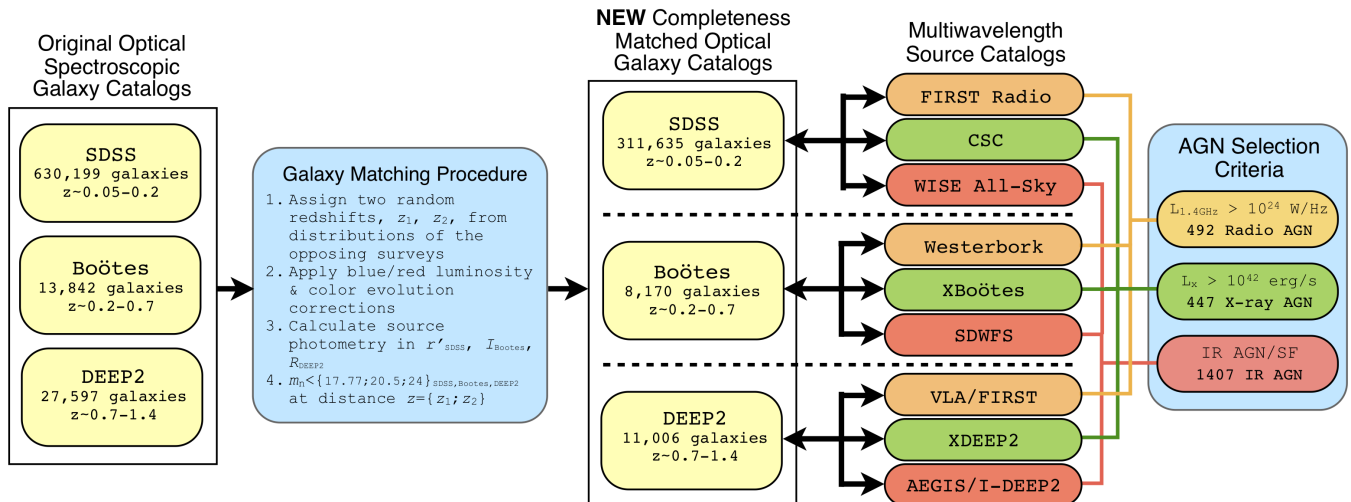
FIG. 1.— A schematic flow diagram highlighting the main steps in the construction of our relatively unbiased, optical-property matched galaxy sample derived from the main SDSS-DR7, Boötes and DEEP2 optical spectroscopic catalogs. Furthermore, we connect our matched galaxy sample, in each survey, to the appropriate multi-wavelength catalogs to identify those galaxies hosting luminous AGN.
