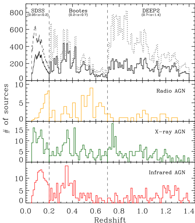
FIG. 2.— Top panel: Spectral redshift distributions for the full parent catalogs (dashed-line; SDSS-MPA-JHU; Kochanek et al. 2012; Newman et al. 2013) as well as the selection and evolution matched galaxy samples (solid line). The final matched galaxy samples contain 311,685, 8,170 and 11,006 sources in SDSS, Boötes and DEEP2, respectively. Lower panels: Spectral redshift distributions for AGN identified at radio (yellow-solid), X-ray (green-solid) and infrared (red-solid) wavelengths in the survey fields. The histograms of the radio and IR AGN in the SDSS are scaled by a factor of 1/10 for presentation purposes.
