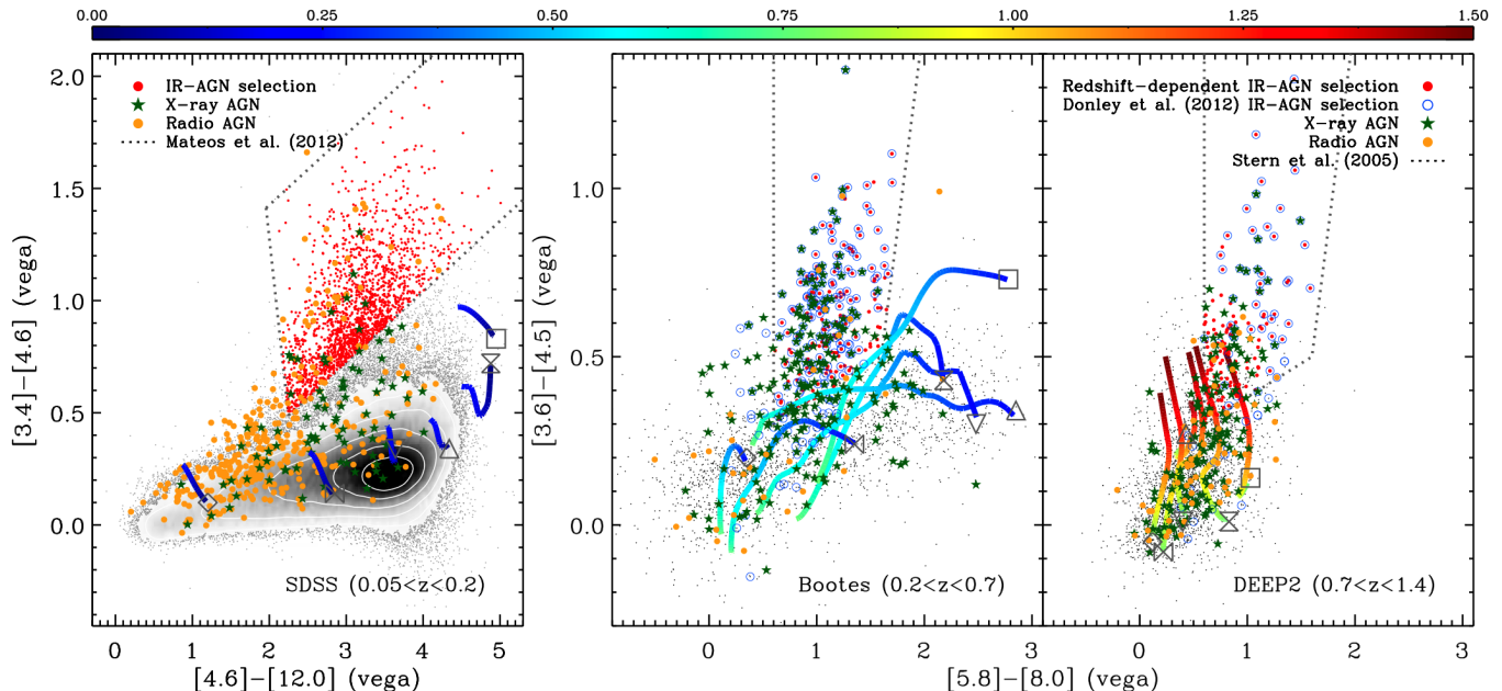
FIG. 3.— Common: Redshift dependent spectral tracks for starburst (square, hourglass), spiral (triangle, upturned triangle, bow-tie) and elliptical (diamond) galaxies are shown. Radio and X-ray detected AGN are shown with orange circles and green stars, respectively. Infrared color-color diagnostic selected AGN are shown with red dots. Our choice of redshift dependent AGN selection regions (see main text) provides a clean AGN sample that does not include star-forming or passive galaxy (non AGN) interlopers. a; left: WISE infrared [3.4]–[4.6] versus [4.6]–[12.0] Vega magnitude color-color selection of galaxies and AGN detected in the SDSS for sources at 0.05 < z < 0.2 (contours and gray dots). The AGN (red circles) lying within the AGN diagnostic selection region of Mateos et al. (2012) is shown with dotted lines. b; center: Spitzer IRAC infrared [3.6]–[4.5] versus [5.8]–[8.0] Vega magnitude color-color selection of galaxies selected in the Boötes survey in the redshift range, 0.2 < z < 0.7 (gray dots). Candidate AGN identified using the Stern et al. (2005; dotted region) and/or Donley et al. (2012; blue open circles) infrared AGN color selection methods are additionally shown. Infrared selected AGN, after removal of star-forming interlopers are shown with red filled circles. c; right: Same as center panel except source sample is derived from the DEEP2 survey at 0.7 < z < 1.4 .
