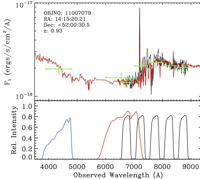
FIG. 8.— Top panel: Example of a typical KCORRECT fit to a DEEP2 galaxy using the measured BR + I'_{1.5} photometry (green points). Flux density as a function of observed wavelength is shown for the DEIMOS spectroscopy (black; Newman et al. 2013), stellar+photoionization+ A_V template produced by KCORRECT is shown with red solid line. Lower panel: Photometric responses for the standard DEEP2 B (blue) and R (red) filters, and our custom narrow I' filters (black) used during the KCORRECT fitting procedure.
