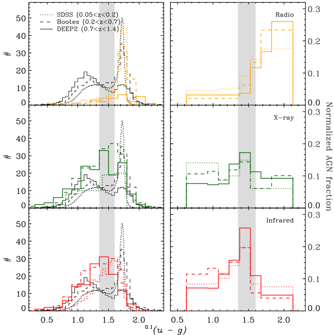
FIG. 6.— Left: Rest-frame ^{0.1}(u-g) color distributions, shifted to z = 0.1 of radio (top panel; yellow), X-ray (middle panel; green) and IR (bottom panel; red) AGN. The respective parent galaxy populations in the SDSS ( 0.05 < z < 0.2 ; dotted line), Boötes ( 0.2 < z < 0.7 ; dashed line) and DEEP2 ( 0.7 < z < 1.4 ; solid line) surveys are shown in black, with the peak values scaled by a factor of 1/40 to match the AGN populations. The approximate position of the ‘green-valley’ is shown in the shaded-region. Right: Same as left panel with AGN histograms normalized to the respective parent galaxy populations. AGN dominated by mechanical energy output are invariably hosted in red massive systems, and are anti-correlated with the hosts of radiatively efficient IR AGN; i.e., IR AGN are hosted in star-forming blue galaxies. When normalized for the underlying parent populations, we find little or no evidence for evolution in the host-galaxy color distributions within the last 9 Gyrs.
