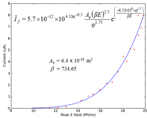
Figure 4: Example of dark current measurement.
