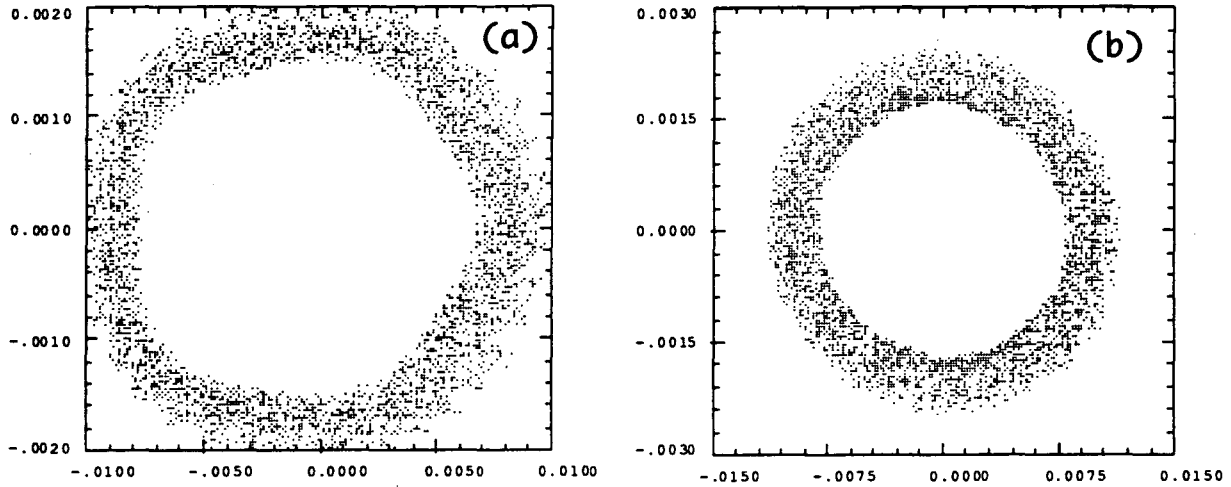
Figure 2: Phase space plots with 6-th order nonsymplectic Runge-Kutta integrator. (a) and (b) are x - p_x and y - p_y plot for 15 integration steps which is equivalent to 120 function evaluation.
