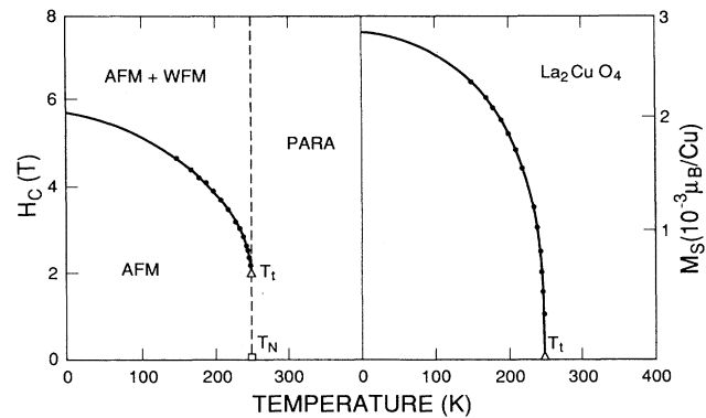
FIG. 3. The left panel: Field-temperature phase diagram deduced from magnetization measurements ( T_N = 253 \pm 0.5 \text{ K} , T_t = 251.5 \pm 0.5 \text{ K} ). The right panel: M_s vs temperature, where M_s is the jump in isothermal magnetization curves.
