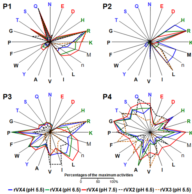
Figure 3. Substrate specificity profiles of vivapains against a tetrapeptide library. A P1 diverse library, and P2, P3, and P4 sublibraries of the P1-lysine fixed library were used to determine specificities. Activities at the four positions (P1, P2, P3 and P4) were compared and are displayed as percentages of the maximum for each position by radial plot. AAs are arranged counter-clockwise from angle zero in decreasing order based on activity of VX-4 at pH 7.5. AAs are represented by the single-letter code (n is norleucine). The representative result of three independent experiments is shown. Black, hydrophobic; Red, acidic; Blue, uncharged polar; Green, basic. doi:10.1371/journal.pntd.0000849.g003
