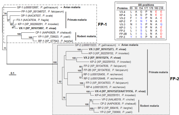
Figure 1. Phylogenetic analysis of malaria cysteine proteases including VX-4. The phylogeny was based on the AA sequence alignment of mature regions. Divergence rates were calculated with the Jones-Taylor-Thornton (JTT) substitution model, and the tree was constructed using the neighbor joining algorithm. The tree was rooted with GP-1 of Plasmodium gallinaceum , which was taken as an out-group. The number at each of the branching nodes indicates the likelihood (percentage) of its appearance in the bootstrapping analysis with 1000 replicates. The enzymes from P. vivax are in bold. The box indicates AAs found in the S2 pocket of primate plasmodial proteases, with position numbers based on mature VX-4. Red, blue, and black AAs are acidic, uncharged polar and hydrophobic, respectively. Note: The vivax protein with accession no. XP_001615272 was annotated as VX-2 during primary analysis of the whole genome sequence of the P. vivax Sal I strain. The name is changed to VX-4 according to our current result (AAT91956). doi:10.1371/journal.pntd.0000849.g001
