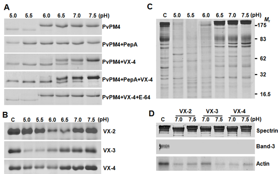
Figure 5. Reactivity of rVX-4 against macromolecular substrates. (A) Processing of P. vivax plasmepsin 4 (PvPM4) by rVX-4. Recombinant PvPM4 (20 \mu g) was incubated with rVX-4 (50 nM) supplemented with 10 mM DTT at different pH values with or without pepstatin A (10 \mu M) or E-64 (1 \mu M) for 3 h at 37°C. The reactants were analyzed by 12% SDS-PAGE. (B) Comparison of hemoglobinolytic activity of VX-2, VX-3 and VX-4. Native human hemoglobin was incubated with the respective enzymes in appropriate buffers (pH ranges 5.0–7.5) supplemented with 1 mM GSH for 3 h at 37°C, after which resolved by 10% SDS-PAGE. (C) Hydrolysis of erythrocyte membrane proteins by rVX-4 at different pHs. Fresh erythrocyte ghosts were incubated with rVX-4 in appropriate buffers (pHs 5.0–7.5) for 3 h at 37°C and reaction products were analyzed by 10% SDS-PAGE. Molecular masses in kDa are shown to the right. (D) Western blotting of erythrocyte ghost proteins. The reactions were done at pH 7 and 7.5. The reactants were separated by 10% SDS-PAGE, transferred to a PVDF membrane and probed with specific antibodies against human erythrocyte spectrin (1:500), band 3 (1:30000) and actin (1:1000) followed by horseradish peroxidase conjugated anti-human IgG (1:1000). The blots were developed with 4C1N. C, control without enzyme.
