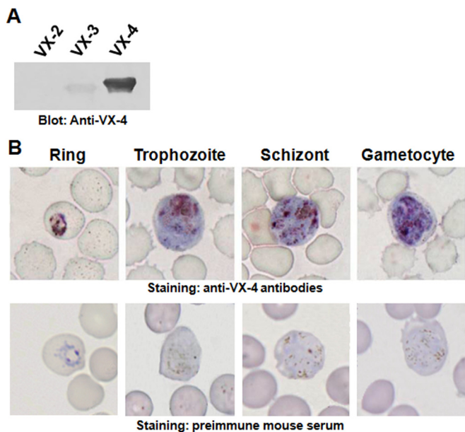
Figure 6. Spatiotemporal Localization of VX-4 by immunocytochemical staining. (A) rVX-2, rVX-3 and rVX-4 proteins were separated by 12% SDS-PAGE and transferred to PVDF membrane. The membrane was incubated with anti-rVX-4 (1:1000 dilutions) for 4 h, with an additional incubation with peroxidase-conjugated anti-mouse IgG (1:2000 dilutions) for 4 h. The blot was developed using 4C1N chromogen. (B) A thin blood smear from a patient with vivax malaria was stained with anti-rVX-4 conjugated with avidin-biotin complex system. The protein was densely labeled in the food vacuoles and adjacent areas, as compared to the staining of the dark hemozoin pigment. doi:10.1371/journal.pntd.0000849.g006
