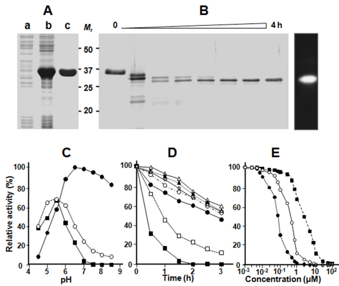
Figure 2. Biochemical properties of recombinant VX-4. (A) Expression and purification of rVX-4. Proteins were analyzed by 12% SDS-PAGE and stained with Coomassie blue. Lanes a, uninduced E. coli lysate; b, IPTG-induced E. coli lysate; c, Ni-NTA purified rVX-4. M_r , molecular masses in kDa. (B) Processing of the refolded rVX-4. The purified rVX-4 was refolded and activated, and aliquots collected every 30 min were analyzed by 12% SDS-PAGE with Coomassie staining (left). The proteolytic activity of fully processed rVX-4 was analyzed by a gelatin gel-zymogram (right). (C) Determination of pH optimum. The VX-4 enzyme activity was assayed in 100 mM sodium acetate (pH 4.5–5.5), sodium phosphate (pH 6.0–6.5) or Tris/HCl (pH 7.0–8.5), each supplemented with 10 mM DTT. Activity was measured at 37°C each against Z-FR-MCA (■), Z-LR-MCA (○), and Z-RR-MCA (●). Maximal activity was presented as 100%. (D) Determination of enzyme stability. rVX-4 was incubated at different pHs in the respective buffers as in panel C. Residual activity was assayed with Z-LR-MCA in 100 mM sodium acetate (pH 5.5) supplemented with 1 mM DTT after indicated incubations at pH 4.5 (●), 5.0 (○), 5.5 (▲), 6.0 (△), 7.0 (☆), 8.0 (□) and 8.5 (■). (E) Inhibition profile for E-64 was determined by incubating rVX-4 (1 μM) with different concentrations of E-64 in 100 mM sodium acetate (pH 5.5; ●), 100 mM sodium phosphate (pH 6.5; ○) or 100 mM Tris-HCl (pH 7.5; ■) at room temperature for 30 min. Residual activities (%) were determined using Z-LR-MCA as a substrate. doi:10.1371/journal.pntd.0000849.g002
