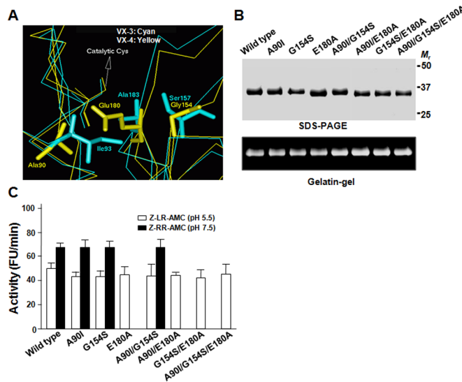
Figure 4. Mutation analyses of VX-4. (A) Superimposition of amino acid residues lining the binding pockets in VX-3 (cyan) and VX-4 (yellow). The residues are shown as sticks and the numbers of residues are indicated in reference to the corresponding pockets/enzymes. (B) Mutagenesis of VX-4. Each mutant was expressed and analyzed by 12% SDS-PAGE (upper) and by a gelatin substrate gel (lower). (C) The activities of wild-type and mutant VX-4s were assayed in 100 mM sodium acetate (pH 5.5) against Z-LR-MCA and 100 mM Tris-HCl (pH 7.5) against Z-RR-MCA at 37°C. In each case, 10 mM DTT was supplemented in reaction buffer. Maximal activity was presented as 100%. Mean \pm S.D. (n=3). doi:10.1371/journal.pntd.0000849.g004
