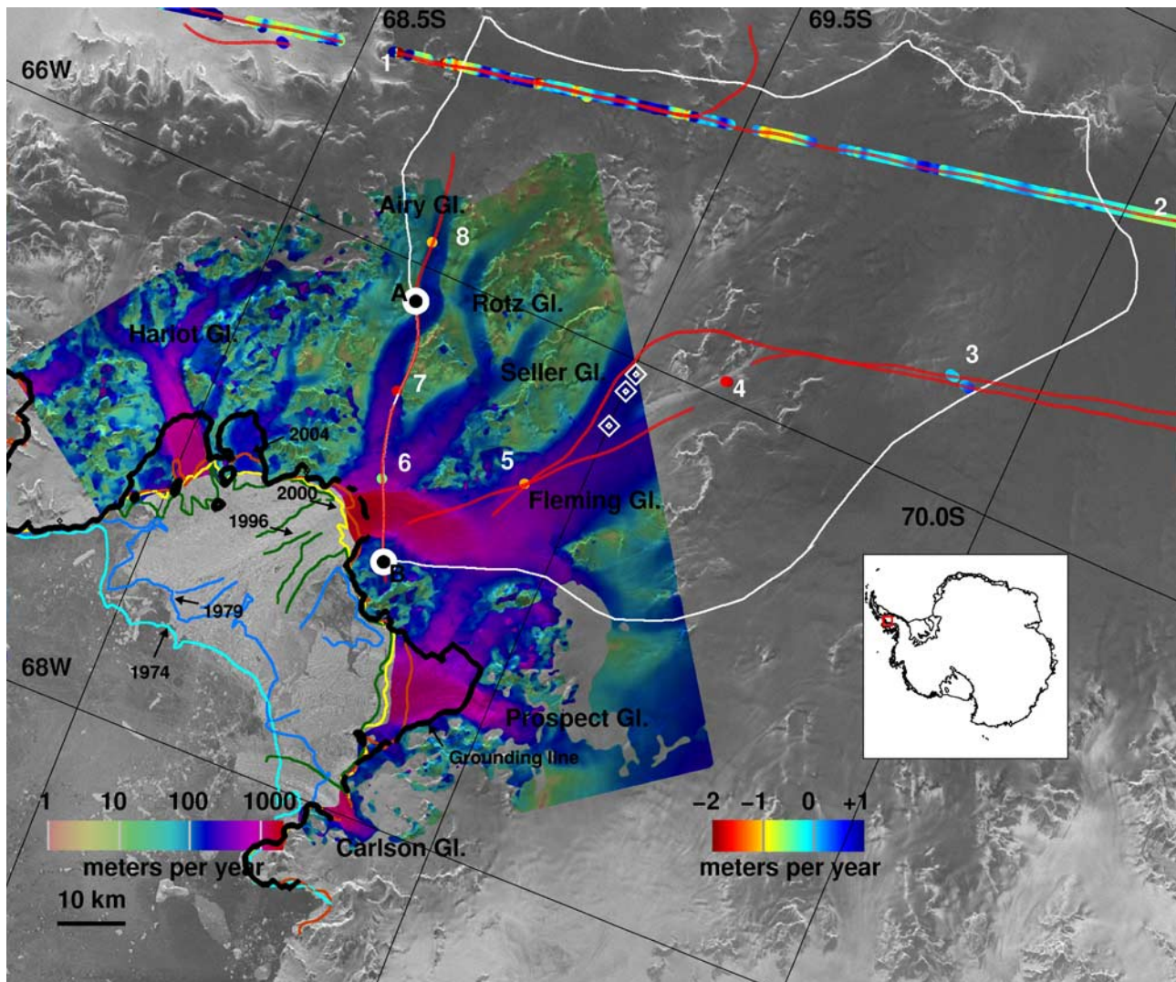
Figure 1. Ice velocity of Hariat, Airy, Rotz, Seller, Fleming, Prospect and Carlson Glaciers from ERS-1/2 1996 and Radarsat-1 2000 interferometry data combined, on a logarithmic scale, overlaid on a radar brightness image of the snow/ice surface [Liu et al. , 1999]. Ice velocities are set to zero beyond the 2000 ice front. Color scale for velocity is on the left, from brown (1 m/yr) to red (>1 km/yr). Grounding line location in 1996 is shown in thick black. Ice front position in 1974, 1979 (Landsat), 1996 (ERS-1), 2000 and 2004 (Radarsat-1) are shown, respectively, in light blue, blue, dark green, yellow and orange. Changes in ice sheet elevation from Nov/Dec 2002 to Sept/Nov 2003 are color coded with the scale on the right, from red (thinning) to blue (thickening). Numbers 1–8 refer to points of thinning quoted in the text. Radar sounding lines are shown in red. Drainage basin is shown in white, extending from the flux gate A-B of Figure 2. In situ velocity measurements by Doake [1975] are white diamonds with a center dot on Fleming.
