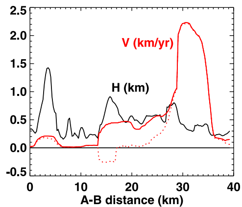
Figure 2. Ice velocity (red is magnitude, dotted red is velocity normal to flux gate) and thickness (black) from CECS/NASA of Airy, Rotz, Seller and Fleming Glaciers along flux gate A-B in Figure 1.
