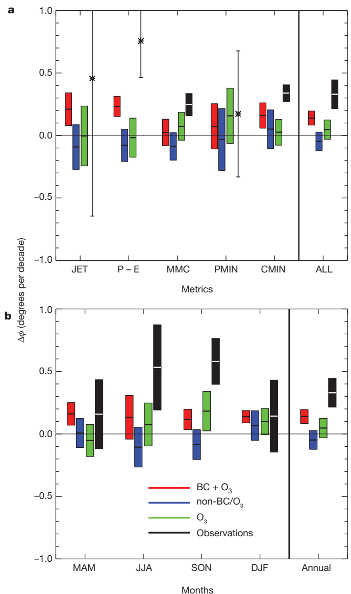
Figure 2 | Observed and modelled 1979–1999 Northern Hemisphere tropical expansion based on five metrics. a , Annual mean poleward displacement of each metric, as well as the combined ALL metric. b , Poleward displacement by season, based on ALL. CMIP3 models are grouped into nine that included time-varying black carbon and ozone (red); three that included time-varying ozone only (green); and six that included neither time-varying black carbon nor ozone (blue). Boxes show the mean response within each group (centre line) and its 2\sigma uncertainty. Observations are in black. In the case of one observational data set, trend uncertainty (whiskers) is estimated as the 95% confidence level according to a standard t -test.
