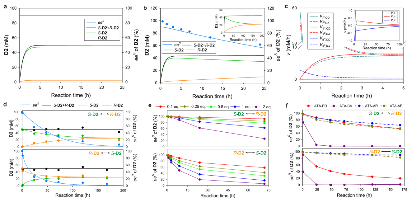
Fig. 3 | Revealing kinetic basis of stereoinversion and demonstrating direct AR reactions by native ATAs. a Kinetic modeling of the ATA-OA reaction in Fig. 2a by considering v_{F,OD} , v_{II^S,RA} , and v_{II^R,RA} only. b Kinetic modeling of the same reaction by additionally including v_{F,RA} , v_{II^S,OD} , and v_{II^R,OD} . Closed circles represent experimental ee^S adapted from Fig. 2a. The inset figure represents the reaction profiles up to 200 h. c Individual rate profiles of OD and RA for I^S , II^S , and II^R for the simulation result of Fig. 3b. The inset figure represents the net rate profiles over an extended
