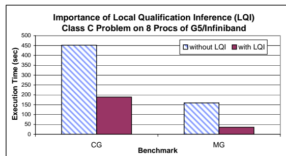
Figure 8: Performance speedup obtained with the LQI compiler optimization
