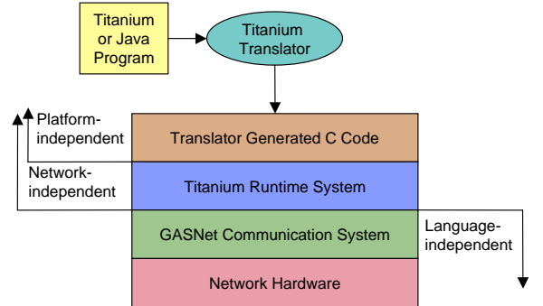
Figure 7: High-level system architecture of the Titanium implementation
