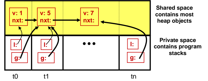
Figure 1: Titanium’s Memory Model.
