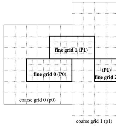
Figure 3: Two levels of an adaptive 2D mesh
