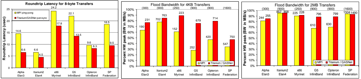
Figure 9: Microbenchmark performance comparison of Titanium/GASNet versus MPI across systems. The latency graph compares the round-trip latency for an 8-byte raw MPI message-passing ping-pong (best case over MPI_Send/MPI_Recv or MPI_Isend/MPI_Irecv) against a Titanium/GASNet blocking put operation (which blocks for the round-trip acknowledgment). Bandwidth graphs show the peak bandwidth at 4KB and 2MB transfer sizes for a unidirectional message flood of the given size, and no unexpected MPI messages. Bandwidth bars are normalized to the hardware peak (a minimum of the I/O bus bandwidth and link speed, as shown in parentheses), and labels show the absolute value in MB/s ( MB = 2^{20} bytes).
