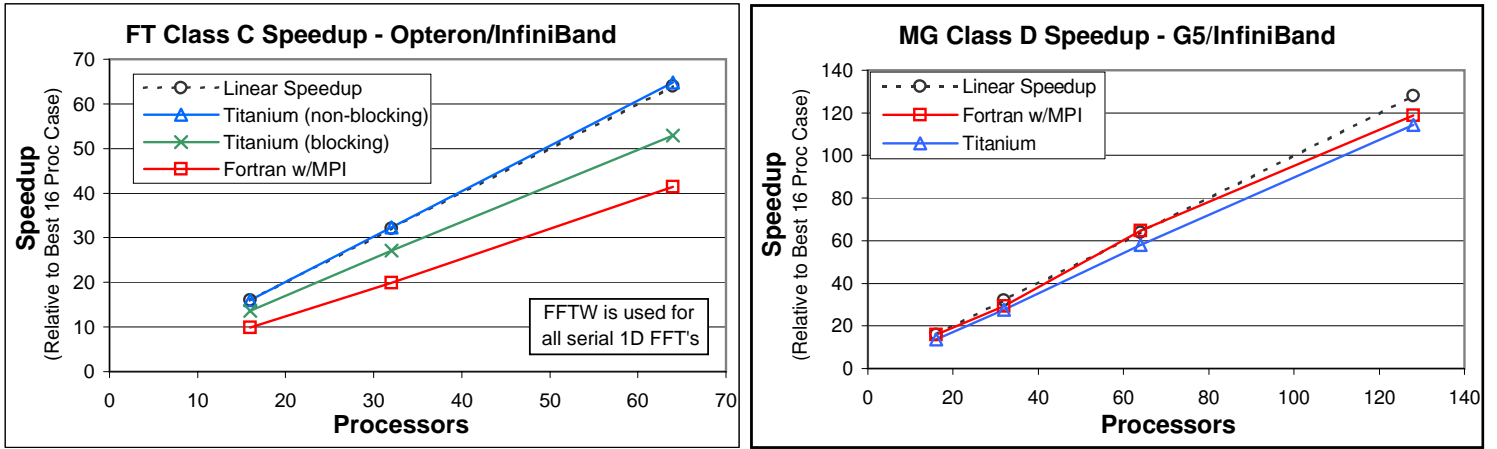
Figure 5: Speedup graphs for NAS FT and MG. The FT benchmark solves a 512^3 problem, while MG solves a 1024^3 problem. All speedups are based on the best time (for either language) at 16 processors.
