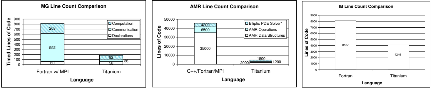
Figure 4: NAS MG, AMR and IB line count comparisons. The Elliptic PDE Solver module of the C++ AMR code has more functionality than the Titanium version and that the Fortran IB version contains only vector annotations but no MPI code or other support for distributed-memory parallelism.
