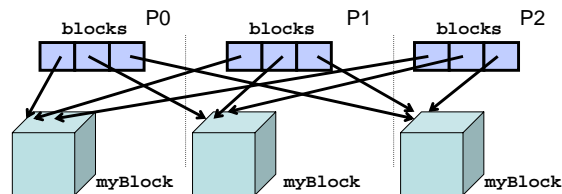
Figure 2: Distributed data structure created by Titanium’s exchange operation for three processors.
