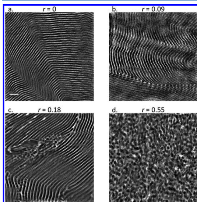
Figure 3. Dark field STEM images of SEO(16–16) at several salt concentrations. Salt concentration increases from (a) through (d). Polymers were stained with \text{RuO}_4 , and PEO domains appear bright. The scale bar in (a) represents 100 nm, and it applies to all images.
