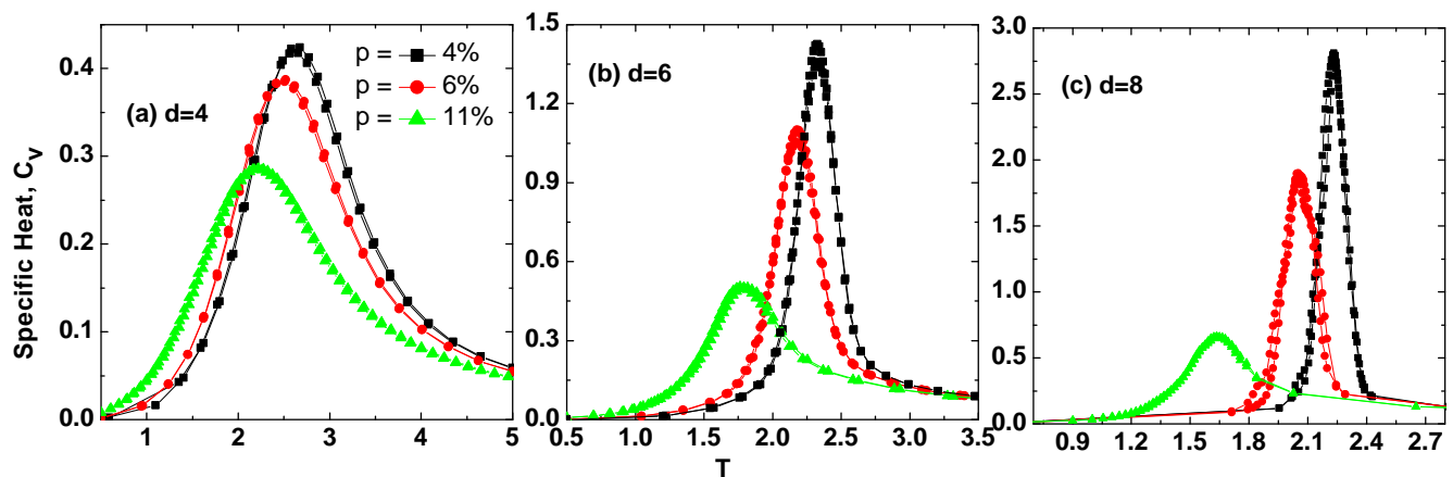
FIG. 3. (Color online) Specific heat C vs. dimensionless temperature T for (3,4) QHP models with distances (a) d = 4 , (b) d = 6 , and (c) d = 8 , at p values as indicated on panel (a). Each curve contains data points from the feedback optimized parallel tempering simulation where ordered and disordered configurations are used as initial states. The peak positions are extrapolated to infinite distance to obtain the transition temperatures, see Fig. 5.
