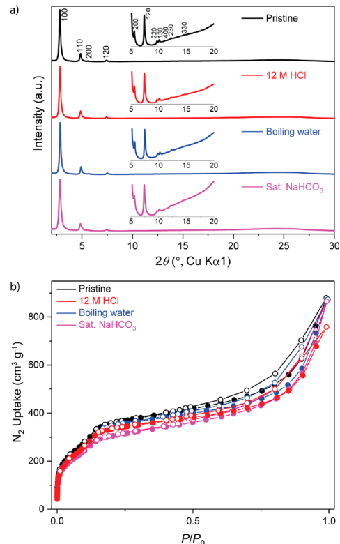
Figure 4. Stability test of COF-118. (a) Comparison of PXRD patterns of methanol-immersed samples. (b) Comparison of N 2 isotherms at 77 K.
