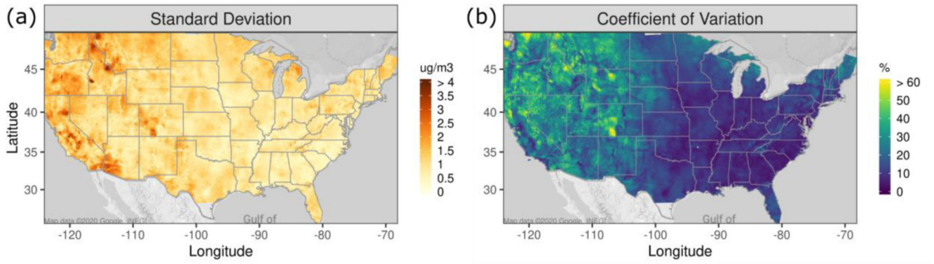
Figure 2. Standard deviation and coefficient of variation for PM 2.5 concentrations from the exposure models in Figure 1, excluding the CTMs (CMAQ and CAMx).
