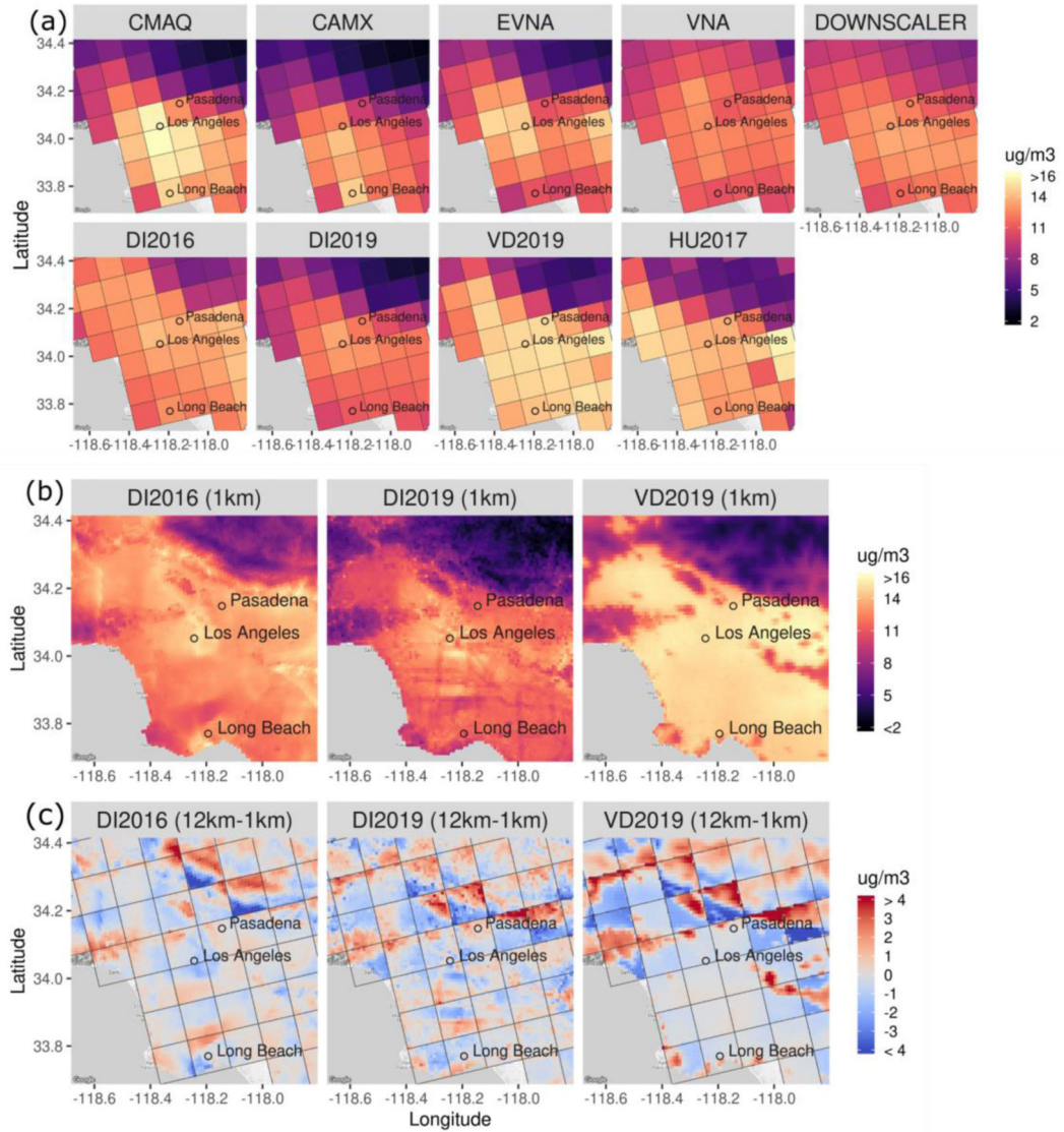
Figure 3. Annual average PM 2.5 concentrations over Los Angeles in 2011 based on (a) 12-km and (b) 1-km gridded exposure fields, and (c) difference between 12-km and 1-km fields (12 km – 1 km).
