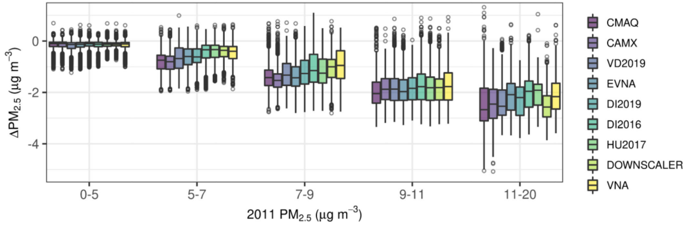
Figure 5. Box and whisker plot depicting distributions of modeled \Delta PM_{2.5} (2028–2011) as a function of 2011 PM_{2.5} concentration. The boxes bracket the interquartile range (IQR; 25th to 75th percentiles), the horizontal line within the box represents the median, whiskers represent 1.5 times the IQR from either end of the box, and circles represent individual values less than and greater than the range of the whiskers, respectively.
