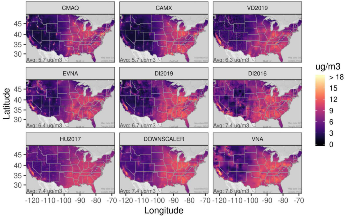
Figure 1. Annual average PM 2.5 concentrations ( \mu\text{g m}^{-3} ) in 2011 based on nine exposure models averaged to a common 12-km grid.
