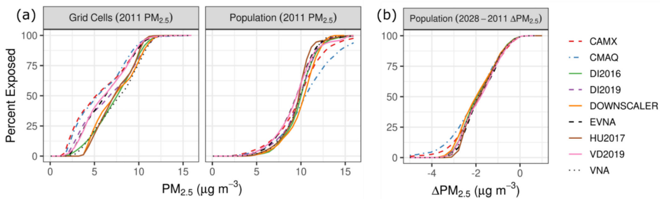
Figure 6. The percentage of (a) U.S. grid cells and population exposed to PM 2.5 concentrations less than the values depicted by the curves and (b) U.S. population exposed to PM 2.5 concentrations less than the values depicted. Population data is based on the 2010 Census.
