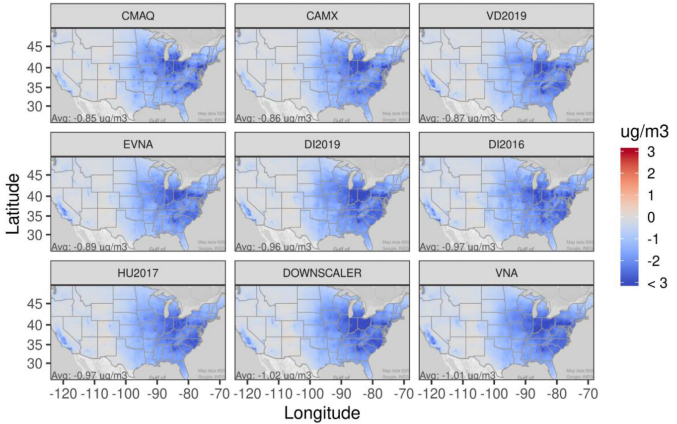
Figure 4. Change in annual average PM 2.5 concentrations (2028–2011; \mu\text{g m}^{-3} ) based on nine exposure models averaged to a common 12-km grid.
