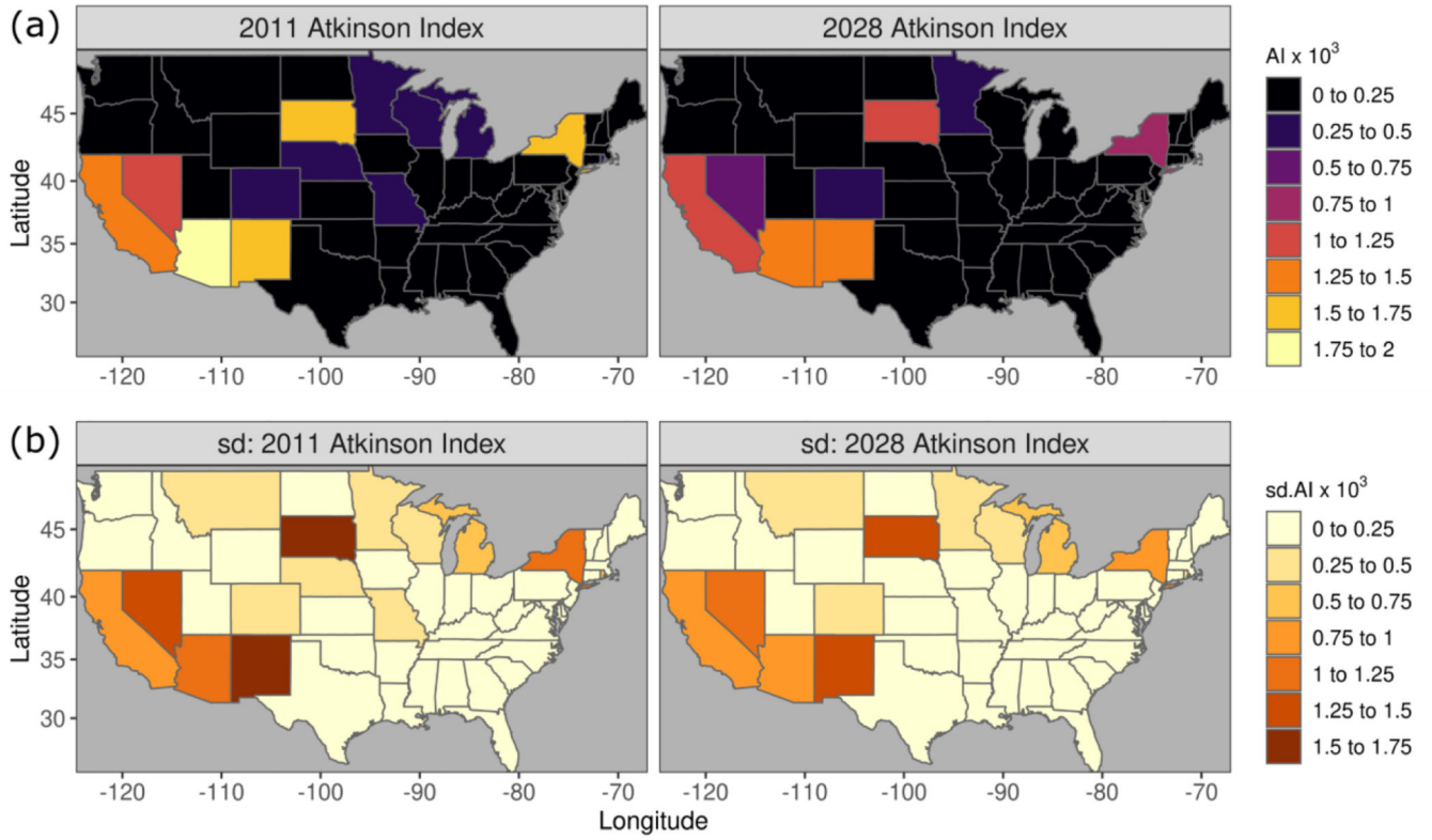
Figure 9. (a) AI_{BG} for 2011 and 2028 based on the mean PM_{2.5} concentrations from the non-CTM models and (b) the sd of the AI_{BG} calculated from the seven non-CTM models.
