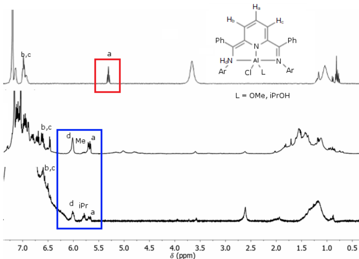
Figure A1 1 H NMR spectrum of (F 5 I 2 P)AlCl(THF) 2 (top), A1 (middle), and A2 (bottom). The labeled chemical structure corresponds to each spectrum. The red box (top) and blue box (middle, bottom) highlight the chemical shifts of the para -pyridyl proton of the ligand and how it changes from the I 2 P 2- ligand charge state to HI 2 P - .
