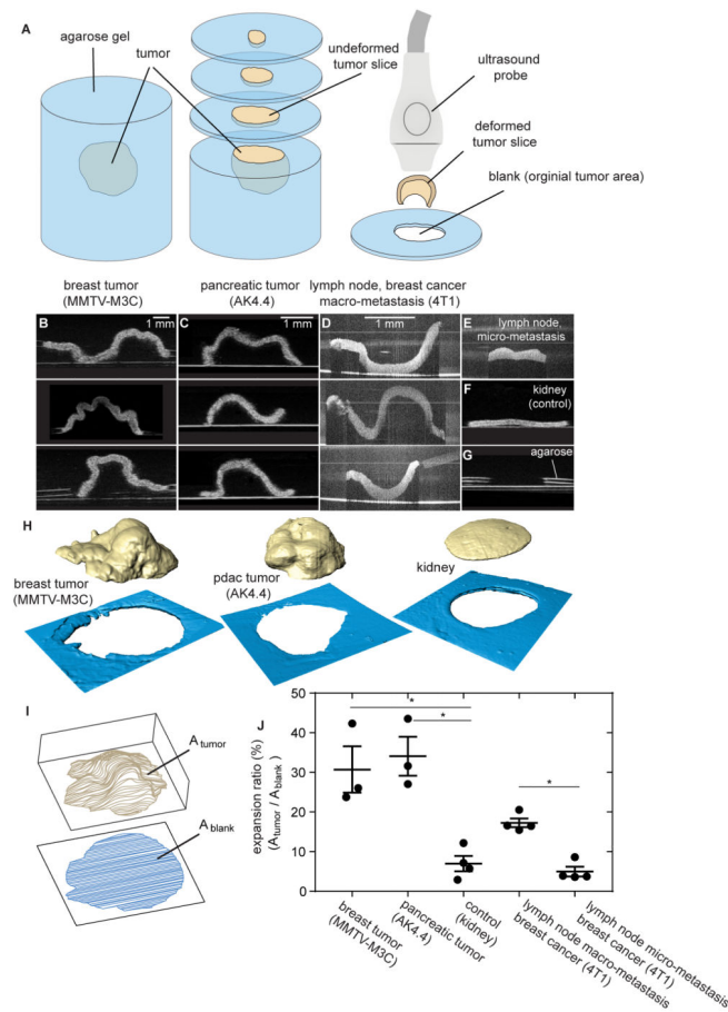
Figure 3. Creating tumour slices provides a sensitive measure of solid stress applicable to a wide range of specimen sizes
