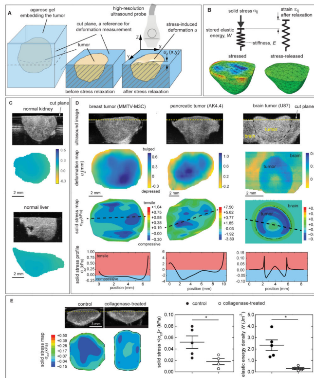
Figure 1. 2-D map of solid stress in tumours
