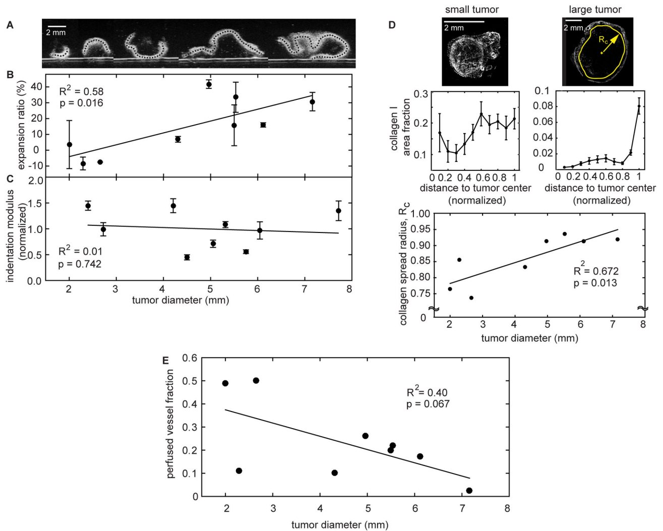
Figure 4. Evolution of solid stress and stiffness as a function of tumour size
