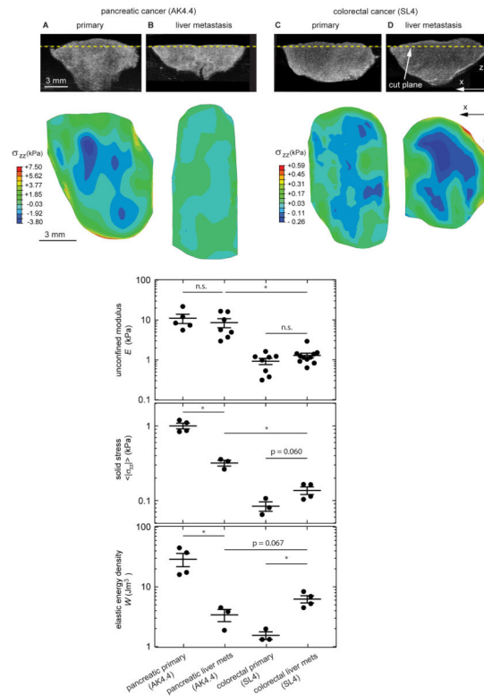
Figure 2. Solid stress and elastic energy in primary vs. metastatic tumours
