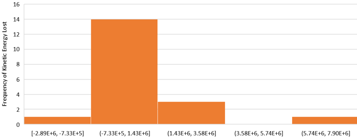
Figure 25. Histogram of the Kinetic Energy lost during braking activity: local route
