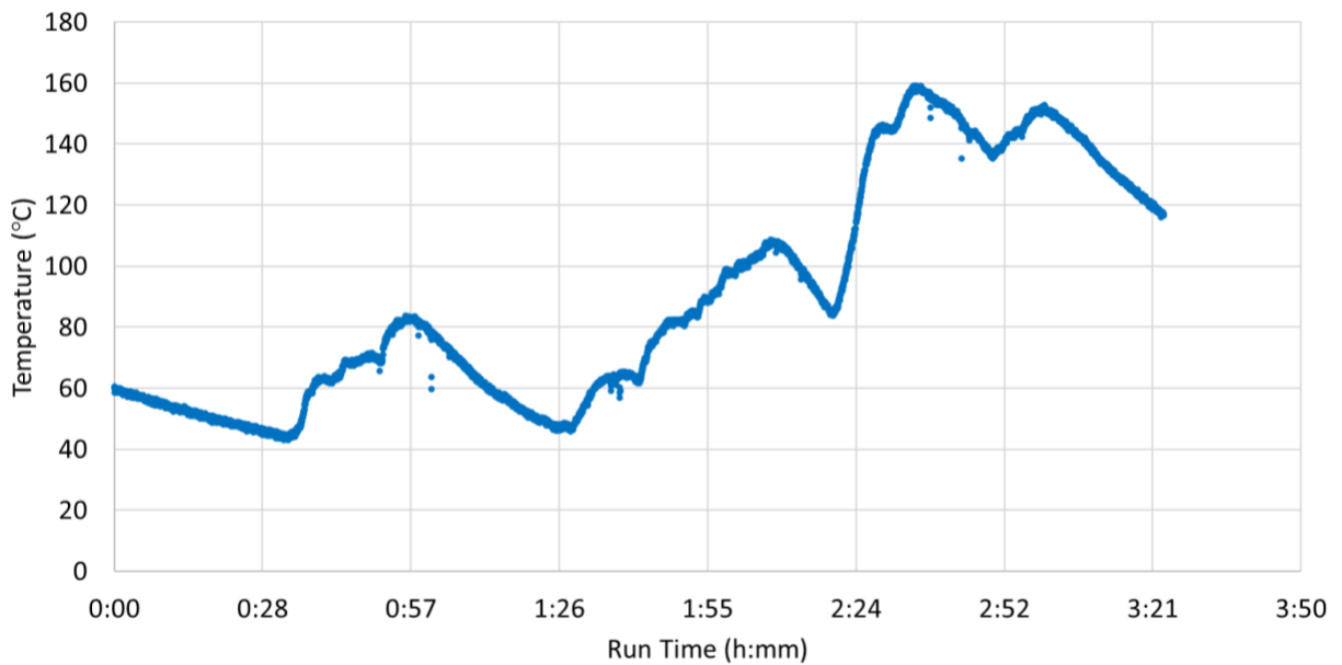
Figure 27. Brake temperature (left rear brake): Freeway route
