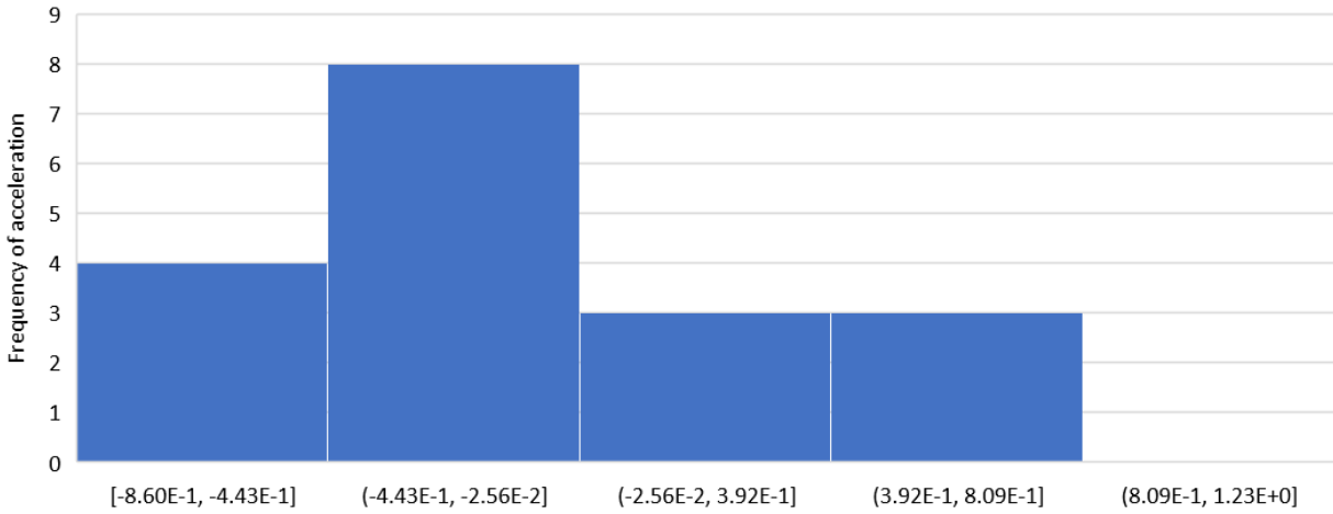
Figure 23. Average acceleration (m/s 2 ) histogram for braking activity: Local
