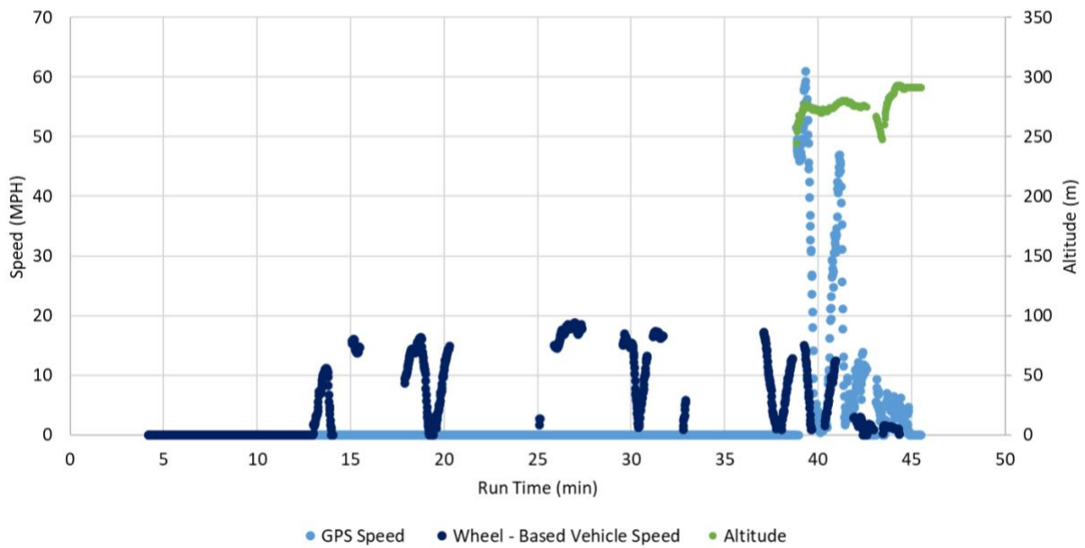
Figure 20. Vehicle speed in MPH and Altitude in meters: Local
