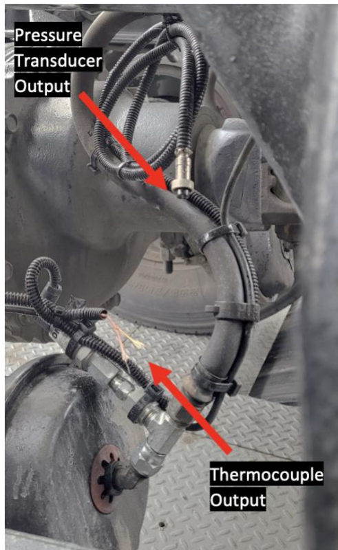
Figure 3. Pressure transducer and thermocouple connections right rear brake-wheel
