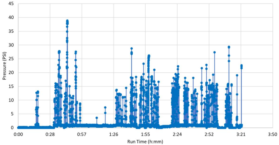
Figure 28. Brake pressure: Freeway route
