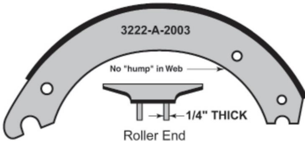
Figure 2. 16-1/2" x 8-5/8" Meritor Q Plus Brake shoe. (Meritor 2018)
