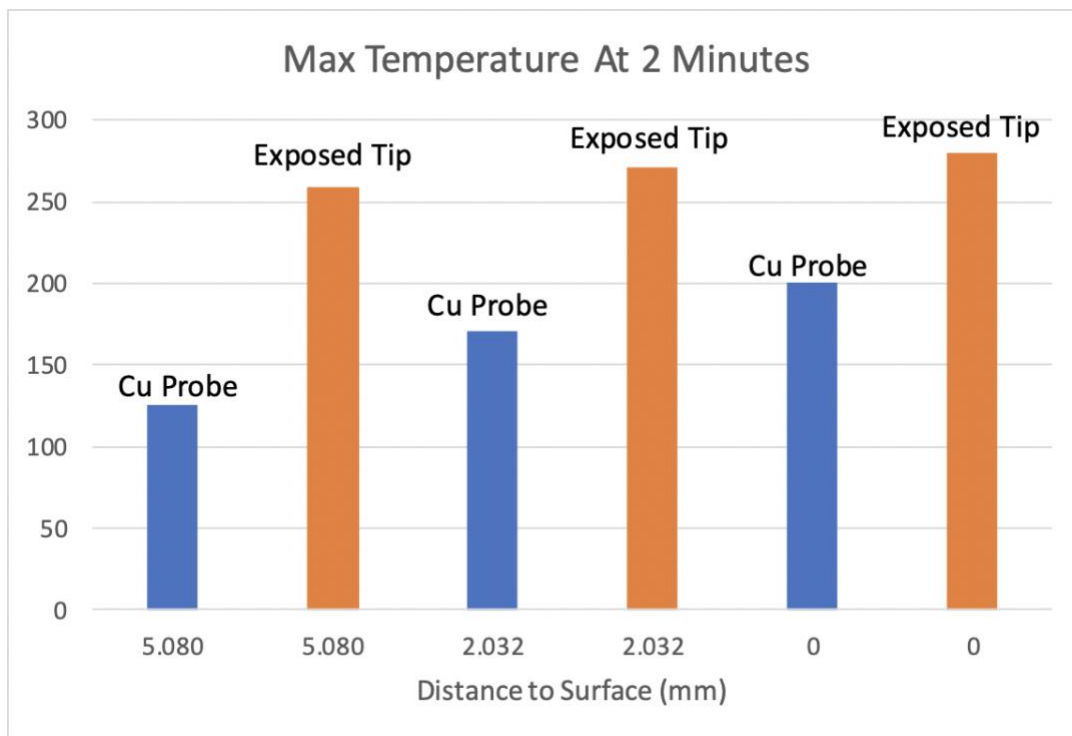
Figure 36. Maximum temperature measured during the 2 min heating cycle for RT plot
