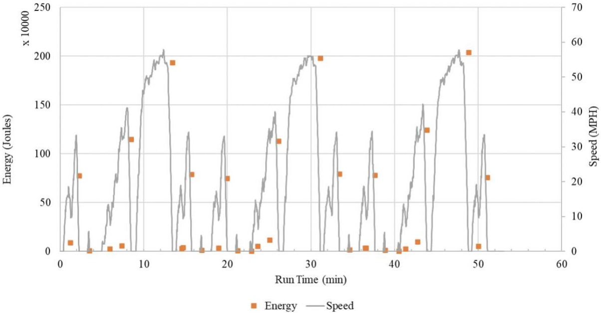
Figure 18. Braking Event Energy: UDDS
