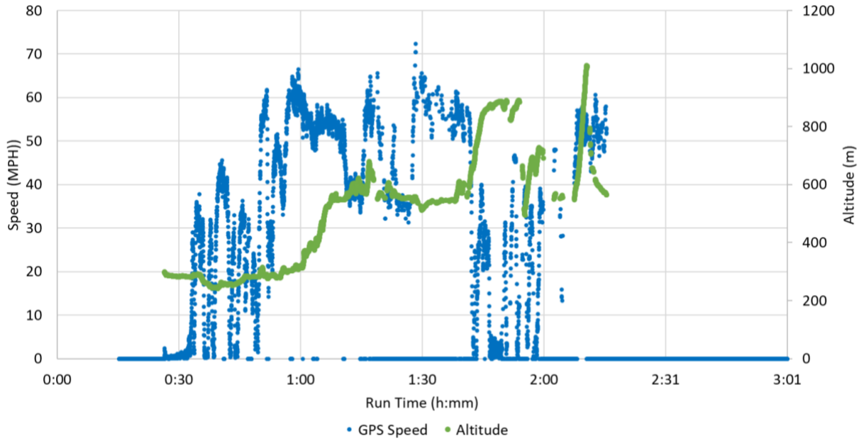
Figure 26. Vehicle speed in MPH: Freeway route
