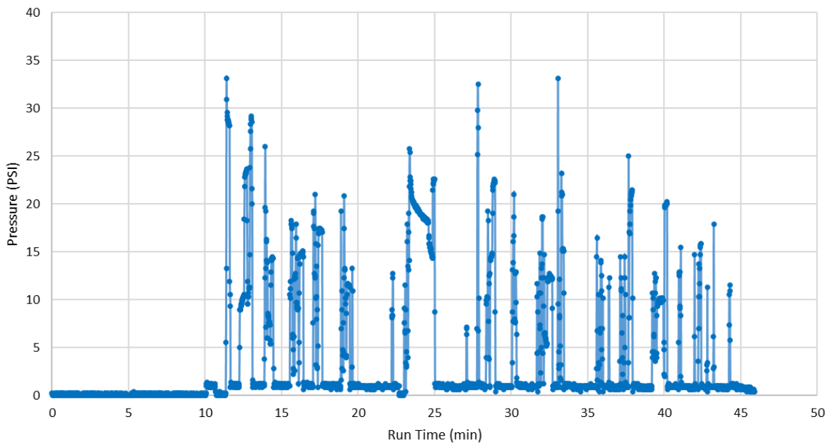
Figure 22. Brake pressure (left rear brake): Local
