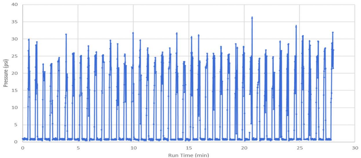
Figure 9. Brake pad pressure (right rear brake): CBD
