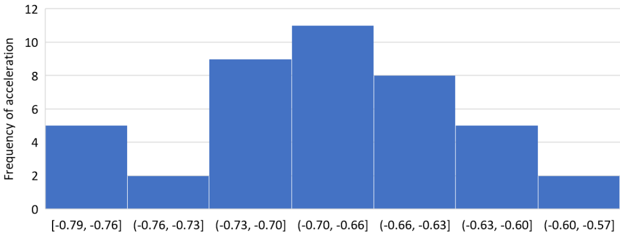
Figure 11. Average acceleration ( m/s^2 ) histogram for braking activity: CBD
