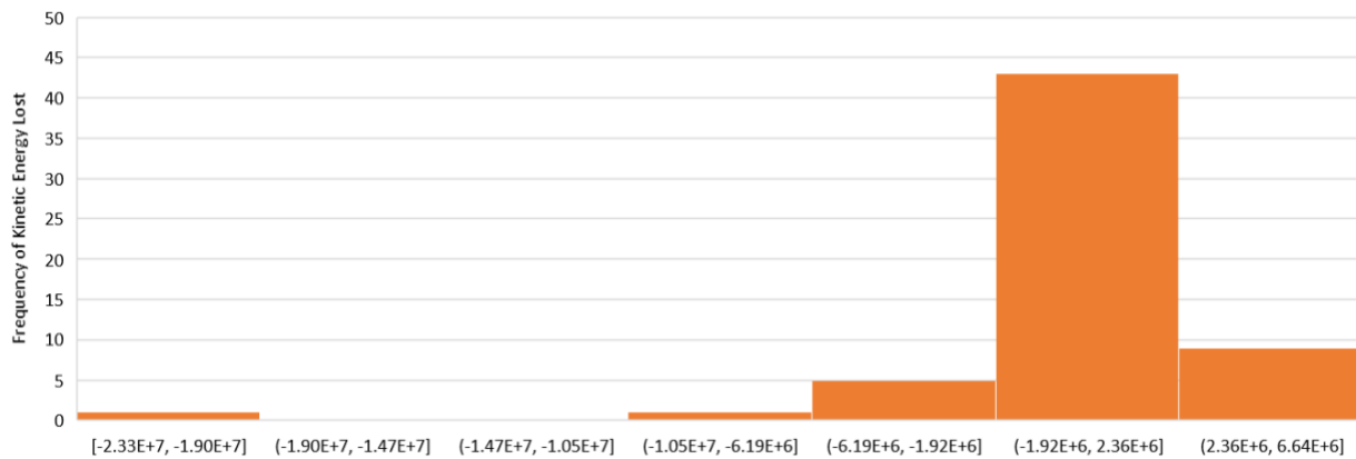
Figure 31. Histogram of the Kinetic Energy lost during braking activity: Freeway route
