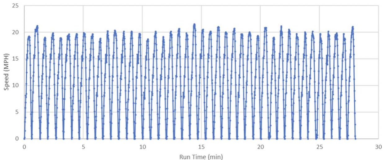
Figure 7. Vehicle speed in MPH for the CBD triplicate test cycle
