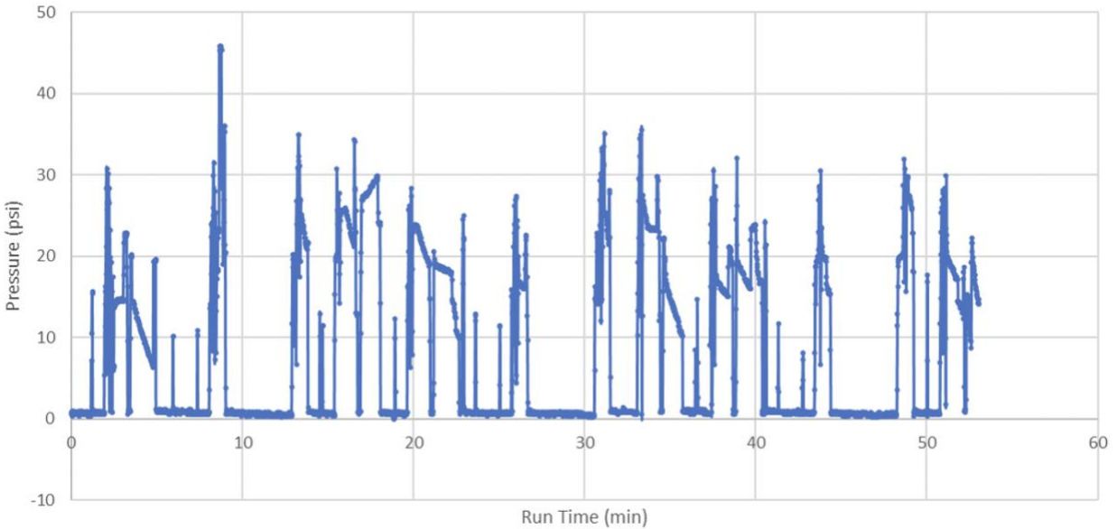
Figure 16. Brake pressure (right rear brake): UDDS
