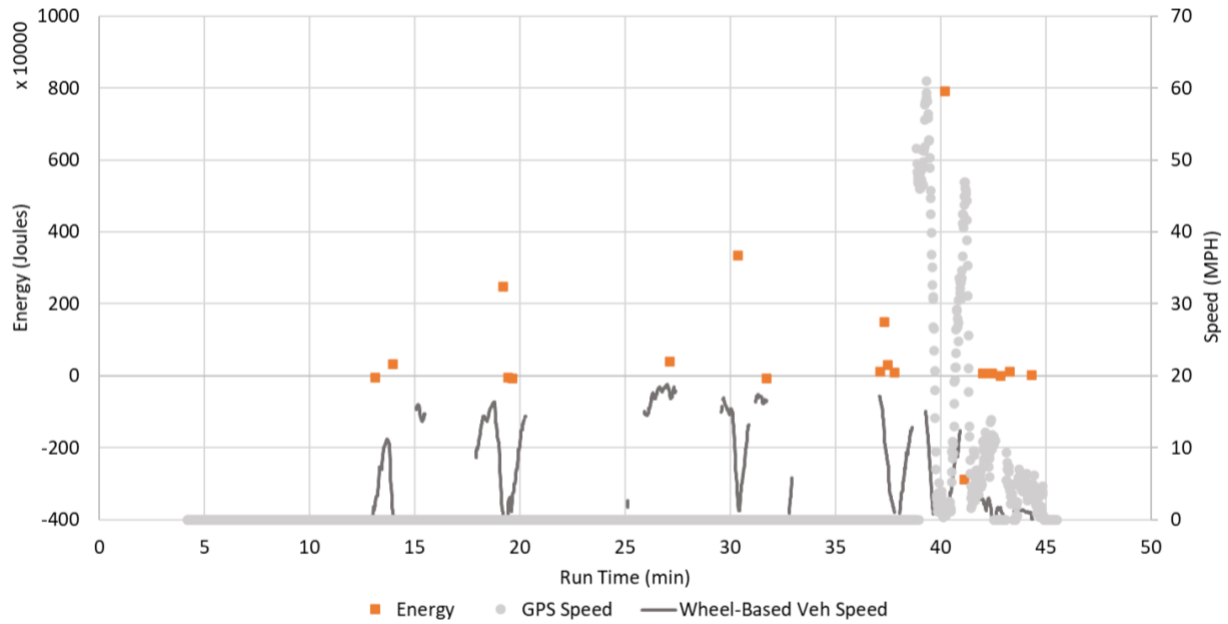
Figure 24. Braking Event Energy: Local
