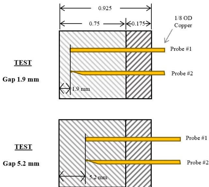
Figure 34. Cross section diagram of thermocouple installation
