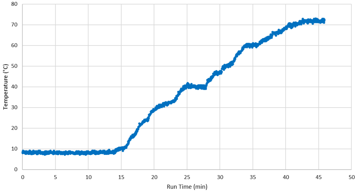
Figure 21. Brake temperature (left rear brake): Local
