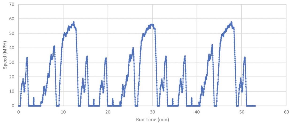
Figure 14. Vehicle Speed in MPH during triplicate UDDS test cycle
