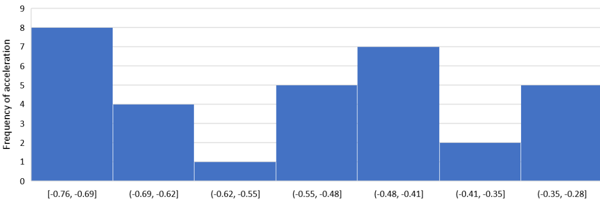
Figure 17. Average acceleration ( m/s^2 ) histogram: UDDS
