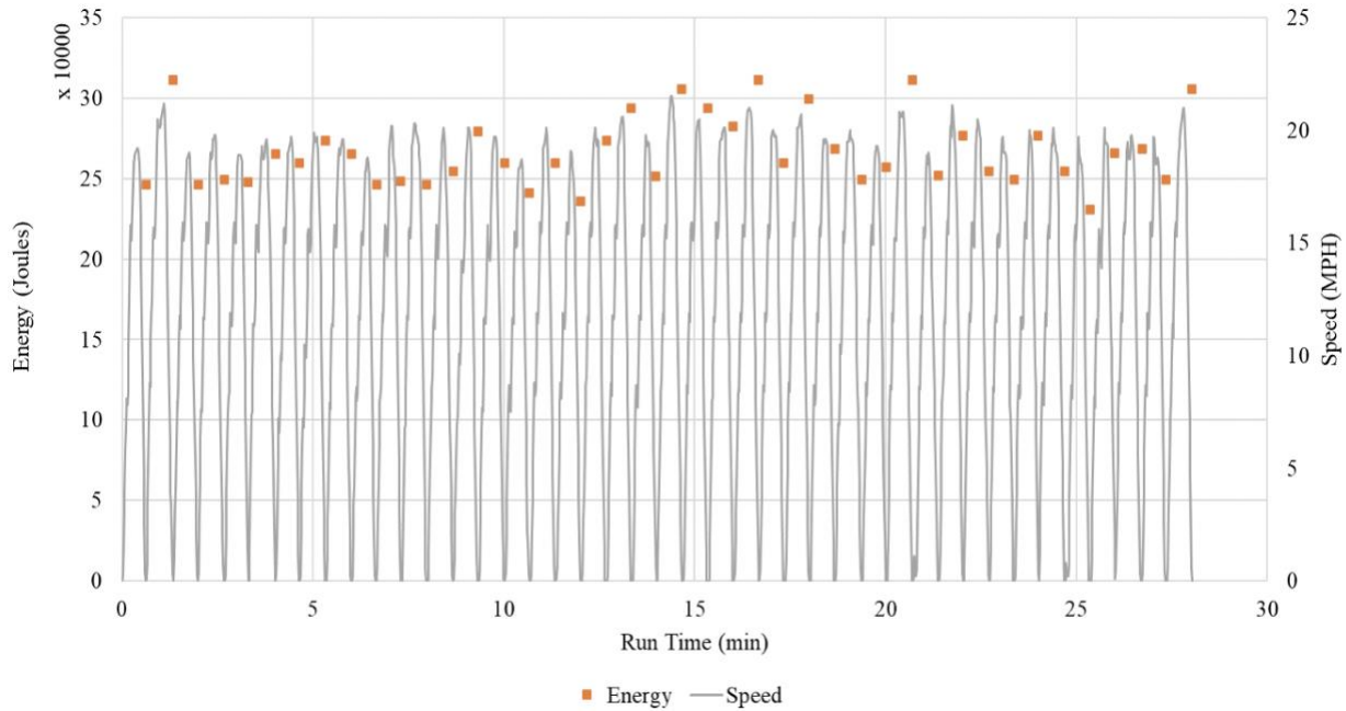
Figure 12. Braking event energy: CBD
