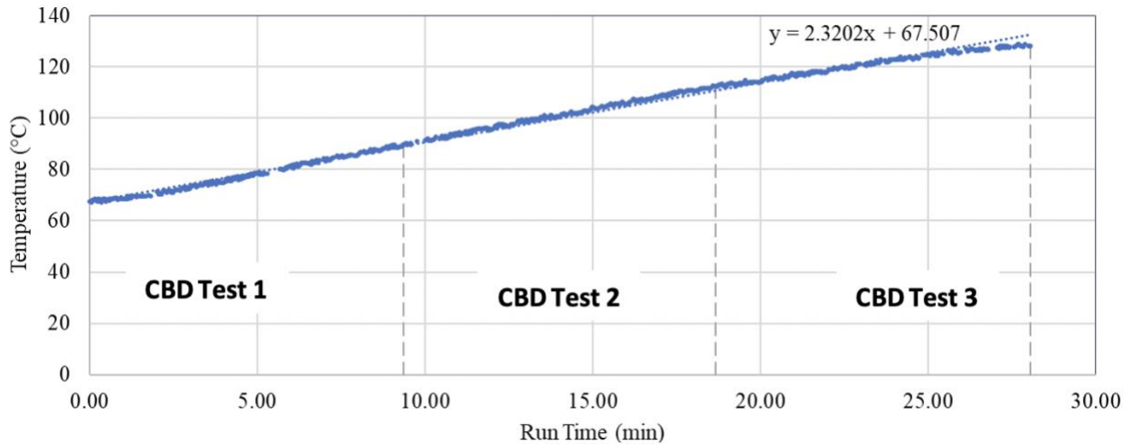
Figure 8. Brake pad temperature (right rear brake): CBD
