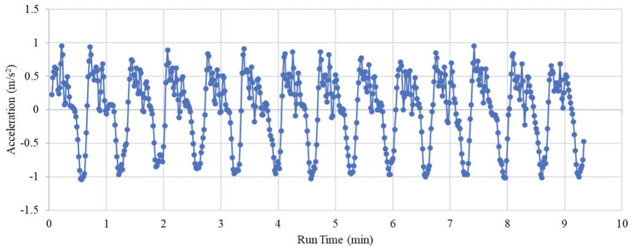
Figure 10. Moving average acceleration ( m/s^2 ) for the 1st CBD cycle
