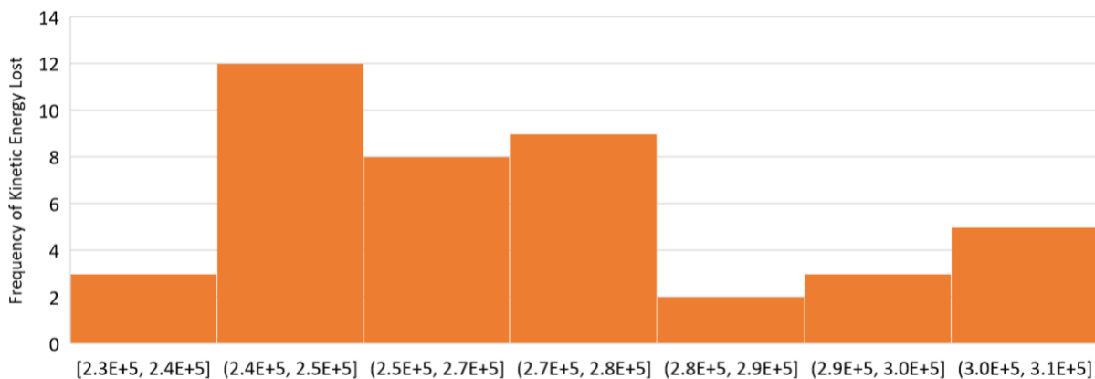
Figure 13. Histogram of the Kinetic Energy lost during braking activity: CBD
