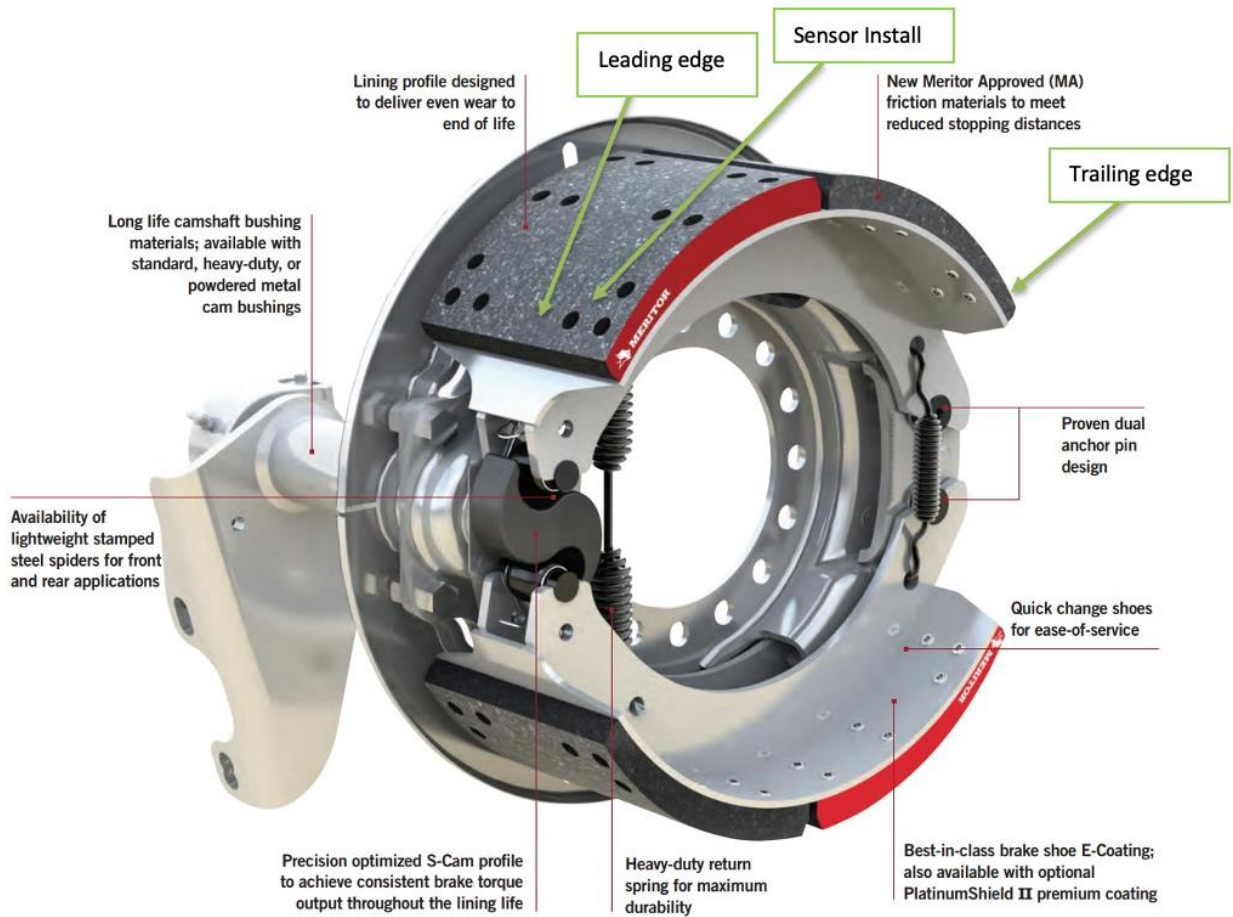
Figure 1. The Meritor Q Plus cam brake system (Meritor 2018)
