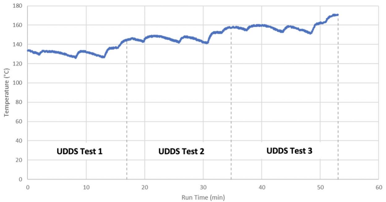
Figure 15. Brake pad temperature (left rear brake): UDDS
