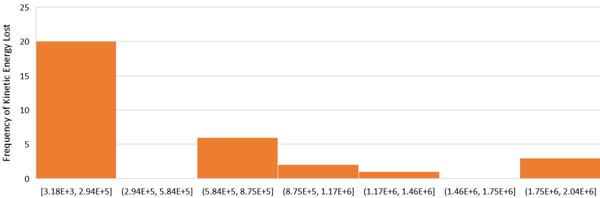
Figure 19. Histogram of the Kinetic Energy lost during braking activity: UDDS
