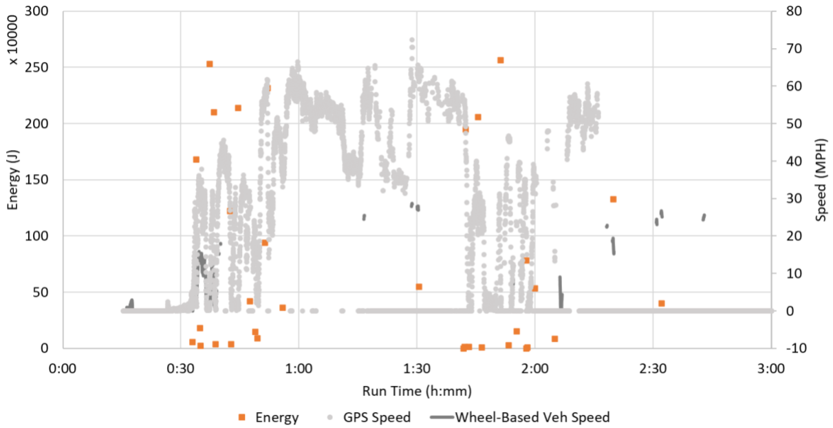
Figure 30. Braking Event Energy: Freeway route
