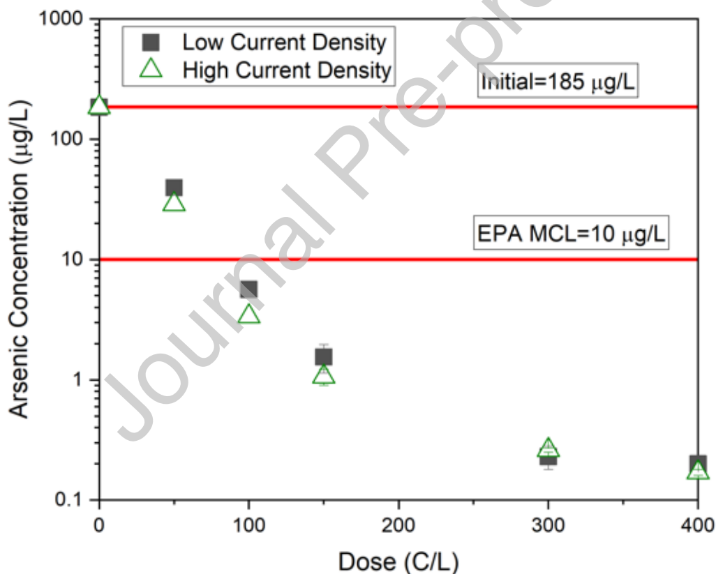
Figure 2 Arsenic concentration ( \mu\text{g/L} ) in the filtered samples at various charge dose (Batches number 3-5). Note vertical scale is logarithmic. All data taken in high conductivity period. Data at 0, 50, 100 C/L are duplicate measurements and everything else is triplicate. Standard deviations are indicated by vertical error bars.
