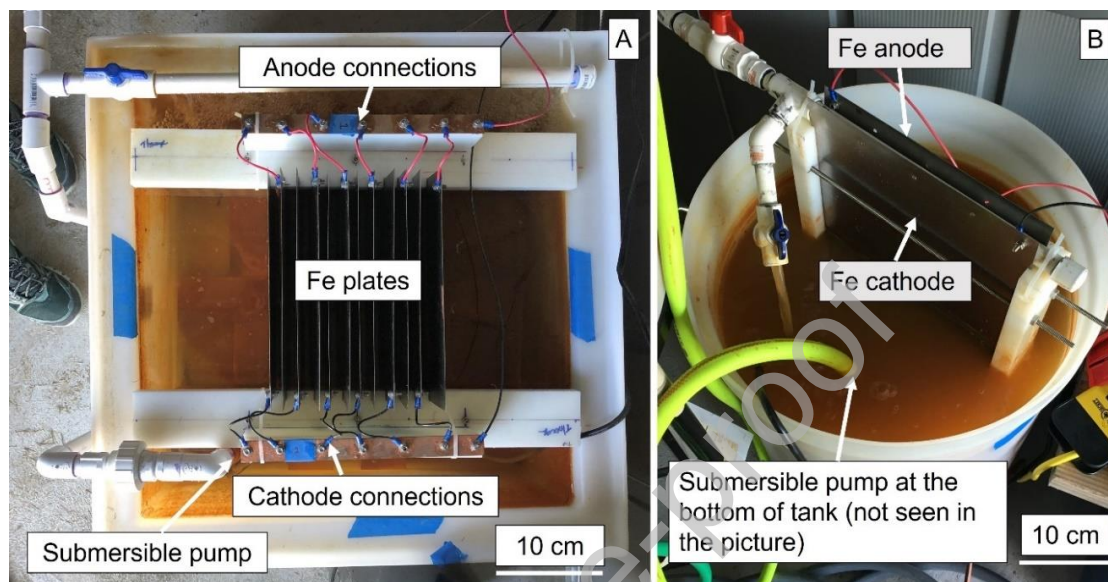
Figure 1 Digital images of the Fe-EC reactors (A- low current density reactor, B- high current density reactor)
