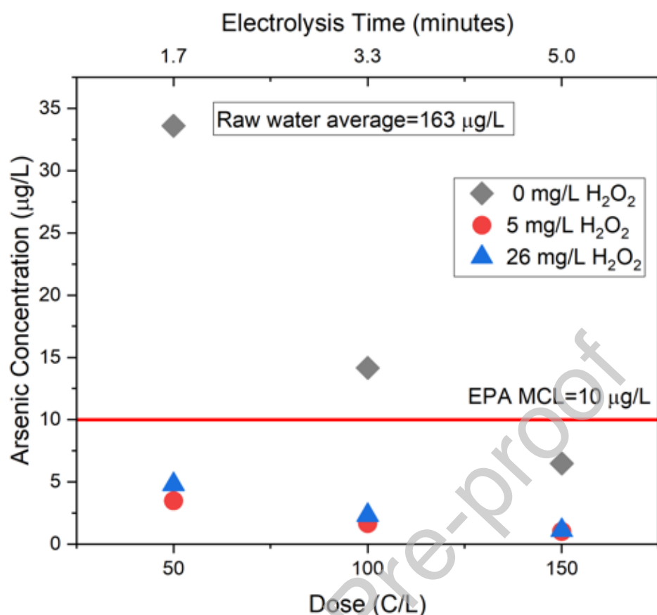
Figure 6 Arsenic concentration ( \mu\text{g/L} ) after electrolysis at varying \text{H}_2\text{O}_2 concentrations (ppm \text{H}_2\text{O}_2 ) and Doses (C/L) (C/L=coulombs/liter) at Dosage Rate of 30 C/L/min. The symbol for 0 mg/L \text{H}_2\text{O}_2 represents a single data point. Those for 5 mg/L and 26 mg/L \text{H}_2\text{O}_2 are the average of duplicates. Time to complete electrolysis to deliver 50 C/L was 1.7 min, 100 C/L was 3.3 min, and 150 C/L was 5 min. The error bars are not shown because they were smaller than the legends.
