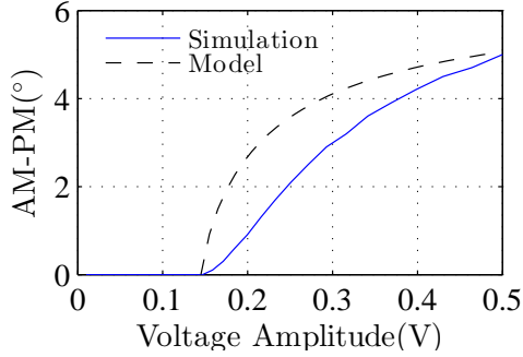
Figure 4.8: AM-PM distortion when R_S = 50\Omega
