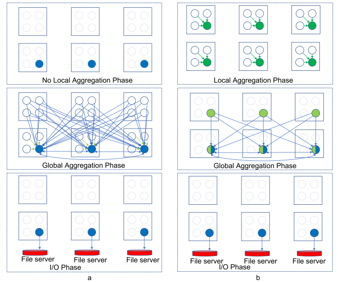
Fig. 2. Illustrations of communication pattern in a collective write operation for two-phase I/O in (a) and TAM in (b). Each square box represents a compute node, and circles are MPI processes. The six green circles are local aggregators, and the three blue ones are global aggregators. Inter-node and intra-node communications are blue and green arrows, respectively. A one-to-one mapping connects the global aggregators and the file servers. In (a), there is no local aggregation phase. The all-to-many (24-to-3) communication pattern shows a potential contention at the global aggregators. In (b), the communication clearly shows a reduced contention (6-to-3) at the global aggregators with the help of local aggregation phase.
