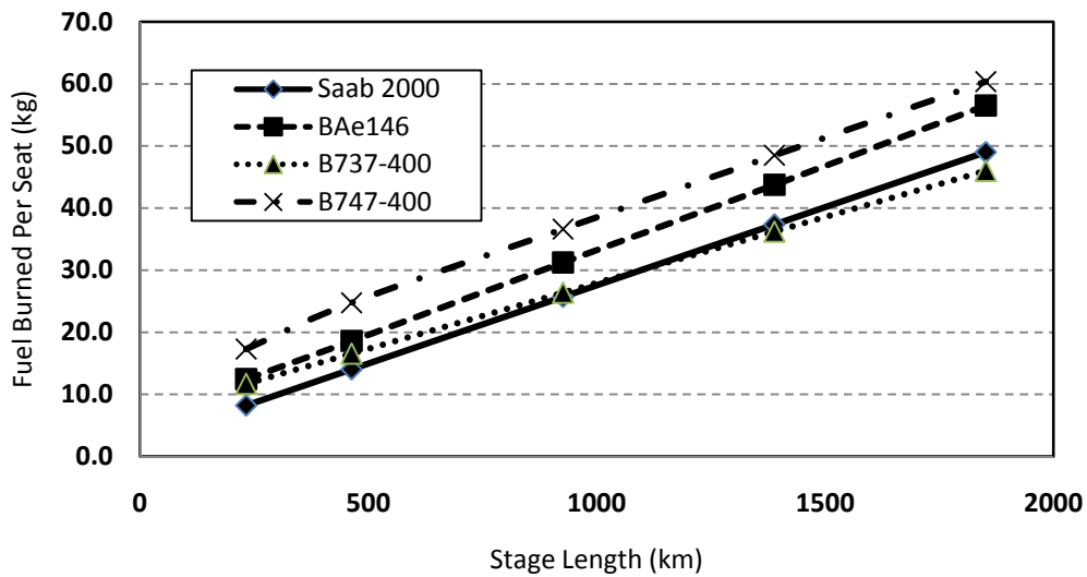
Figure 4 Fuel Burn per Seat vs. Stage Length for Four Representative Aircraft.
