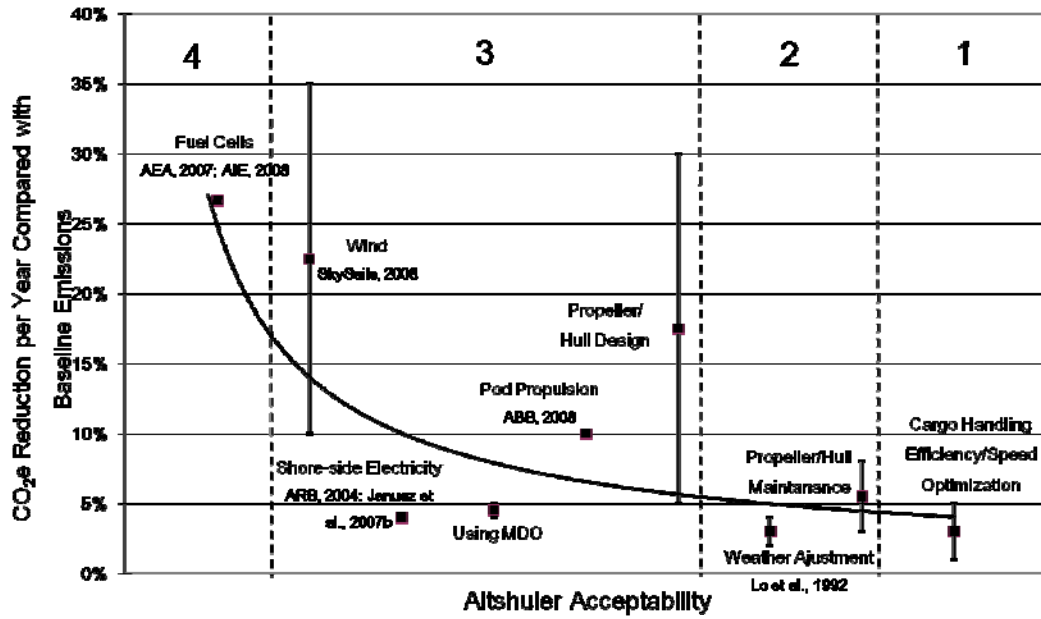
Figure 3 GHG Reduction Potential and Acceptability of Strategies in the Maritime Sector.
