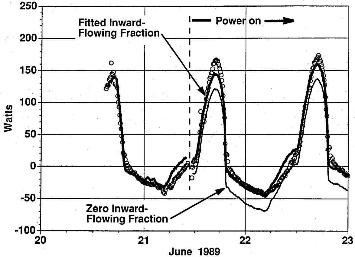
Figure 6. Determination of inward-flowing fraction for an interior shade. The MoWiTT measurement of the apparent net heat flow through the window (open circles) is plotted with the calculated curve for the fitted value of N_i (heavy curve) given by Equation 5. Comparison with the same calculation assuming N_i = 0 (light curve) gives a measure of the significance of the determination. The two curves coincide before the blind was electrically heated. The fact that the model of Equation 5 does not accurately fit the measured points in the morning or near the solar intensity peak is probably related to the assumption of a constant value of F .
