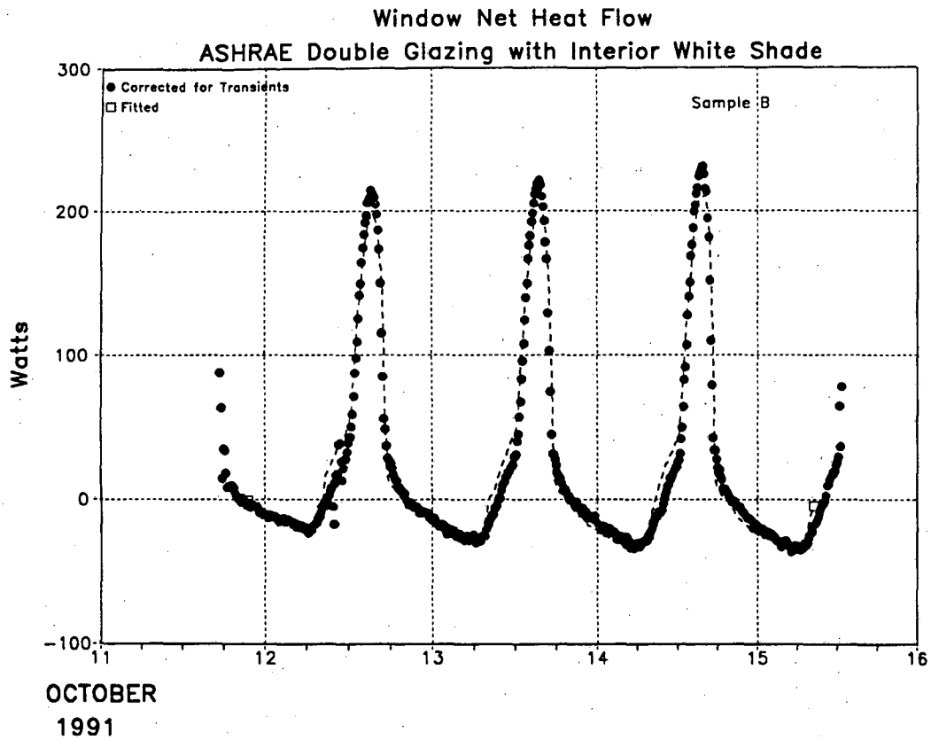
Figure 7. Calorimetric determination of the solar heat gain coefficient for double glazing with an interior white shade. The MoWiTT measurement of the net heat flow through the window (points) is compared to the model of Equation 6 (dashed curve) using the values of the fitted parameters given in the text.
