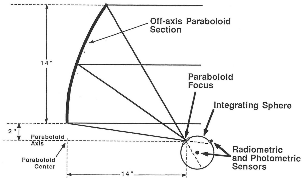
Figure 4. Scanning radiometer detector optical collection system. Light parallel to the axis of the detection system is collected by an off-axis parabolic mirror and focused onto the entrance port of an integrating sphere containing both radiometric and photometric sensors. Radiometric and photometric data are recorded simultaneously. This scheme provides wavelength-independent collection of radiation from a large sample area, combined with a sharp angular selectivity. Wavelength sensitivity is determined by the reflectance characteristics of the integrating sphere interior coating and is good from 350-2200 nm.
