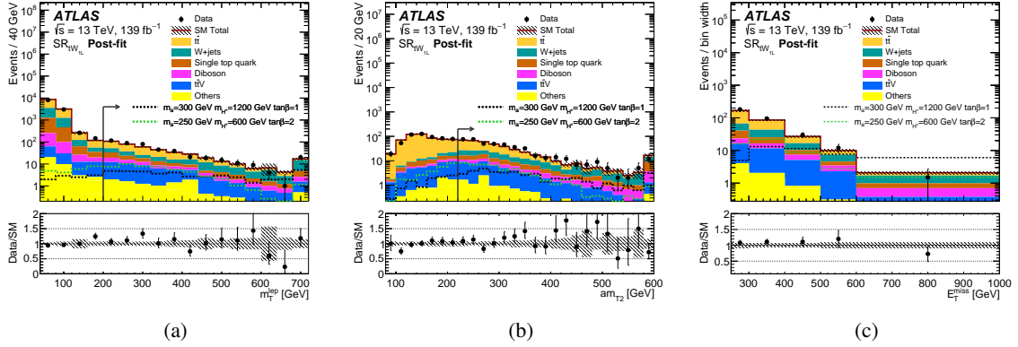
Figure 10: Representative distributions of (a) m_T^{\text{lep}} , (b) am_{T2} and (c) E_T^{\text{miss}} in the tW_{\text{IL}} channel. Observed data are compared with post-fit SM predictions. All SR selections except the one on the quantity shown are applied. The SR requirement is indicated by the arrow. The ‘Others’ category includes contributions from Z +jets and tWZ production, and rare processes such as triboson, t\bar{t}\bar{t} , t\bar{t}WW , and Higgs boson production processes. The expected distributions for representative scenarios with different m_a , m_{H^\pm} , and \tan\beta are shown for illustrative purposes. The overflow events, where present, are included in the last bin. The lower panels show the ratio of data to the background prediction. The hatched error bands indicate the combined experimental and MC statistical uncertainties on these background predictions.
