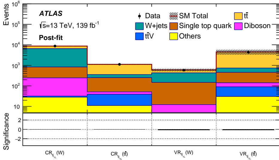
Figure 7: Comparison of the predicted backgrounds with the observed numbers of events in the CRs and VRs associated with the tj_{\text{IL}} channel. The normalisation of the backgrounds is obtained from the fit to the CRs. The upper panel shows the observed number of events and the predicted background yield. The ‘Others’ category includes contributions from Z +jets and tWZ production, and rare processes such as triboson, t\bar{t}t\bar{t} , t\bar{t}WW , and Higgs boson production processes. All uncertainties are included in the uncertainty band. The lower panel shows the significance for each region.
